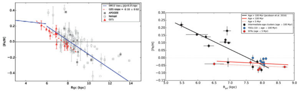
Figure 7. Left: The red filled triangles and dashed line show the radial metallicity gradient defined by the12 Gaia-ESO inner disk ( R_{gc} \leq 8 kpc), intermediate age open clusters (0.2-1.6 Gyr) in internal Data Release 4. The gradient is -0.10 \pm 0.02 dex/kpc. For comparison, APOGEE clusters in Frinchaboy et al. (2013) and the compilation by Netopil et al. (2016) are also shown as grey filled and open squares, respectively. The solid blue line indicates the metallicity gradient in Hayden et al. (2014), based on APOGEE field giants. Right: Radial metallicity distribution of all the Gaia-ESO open clusters and star forming regions (iDR4). Different colours indicate star forming regions (red), young open clusters (blue, age 10-100 Myr), and older clusters (black, intermediate age). The lines indicate the gradient defined by the young clusters (the two red, flattish lines) and by the older clusters (the black, steeper line). Figure adapted from Fig. 2 in Jacobson et al. (2016) and Fig. 5 in Spina et al. (2017), respectively; see the original papers for details.
