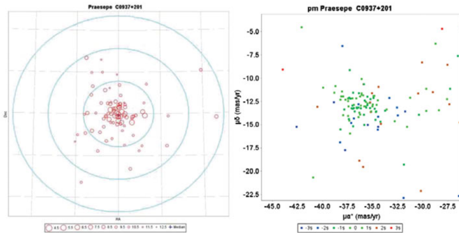
Figure 4. Left: map of the TGAS members of the Praesepe open cluster; the circles are at 5, 10, and 15 pc from the cluster centre, while the grid is at 2 degrees intervals. Right: TGAS proper motions distribution for Praesepe, colour-coded according to difference from the cluster mean parallax. Figure adapted from Figs. D.7 and D.8 in Gaia Collaboration, van Leeuwen, Vallenari, et al. (2017), see the paper for details.
