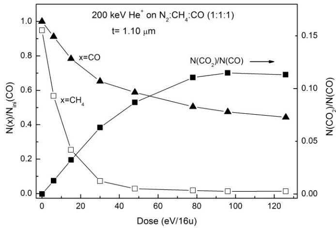
Figure 4. \text{CH}_4 and \text{CO} normalized column densities and \text{CO}_2/\text{CO} column densities ratio of a 200 keV \text{He}^+ irradiated \text{N}_2:\text{CH}_4:\text{CO} (1:1:1) mixture at different irradiation doses.
