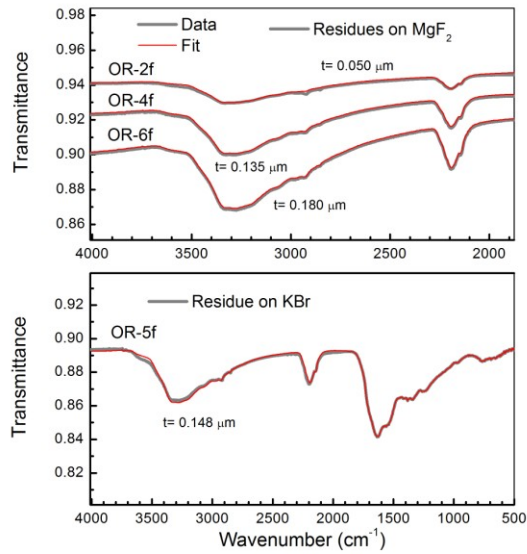
Figure 10. Comparison between theoretical (fit) and experimental average spectra of the organic residues on \text{MgF}_2 and KBr substrates in the IR range. The labels OR-xf indicate the organic residues obtained from x fringes ice films respectively, t is the actual thickness of the residues.
