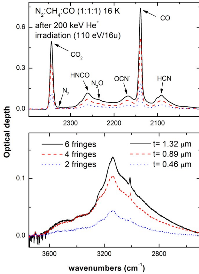
Figure 3. Infrared spectra (16 K) of the icy mixtures \text{N}_2:\text{CH}_4:\text{CO} (1:1:1) after irradiation with 200 keV \text{He}^+ ions (110 eV/16u).
