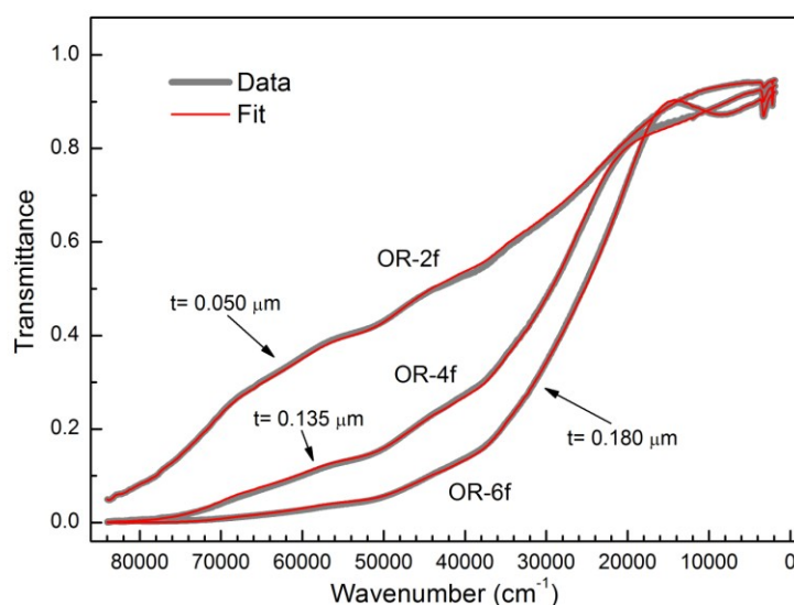
Figure 9. Comparison between theoretical (fit) and experimental average spectra of the organic residues on \text{MgF}_2 substrate. The labels OR- x f indicate the organic residues obtained from x fringes ice films respectively, t is the actual thickness of the residues.
