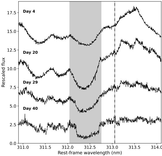
Figure 15. The evolution of the broad absorption feature centered at \lambda = 312.5 nm, marked with a gray shaded region, and attributed to {}^7\text{Be II} 313.0/1 nm doublet. The dot-dashed black line marks the rest-frame position of the {}^7\text{Be II} 313.0 nm line.
