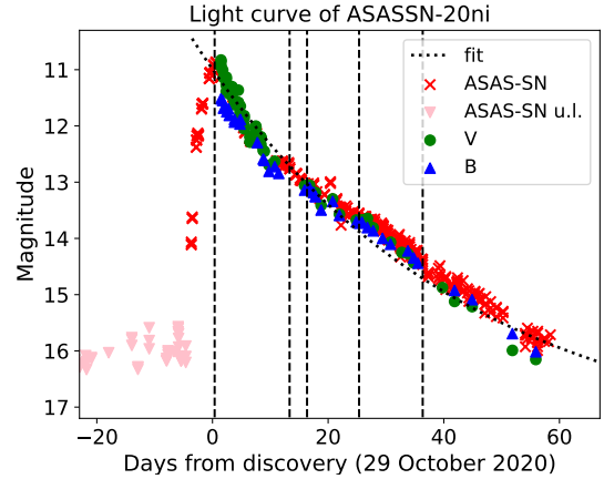
Figure 3. The light curve of ASASSN-20ni as obtained from the AAVSO data archive (Kafka 2021) in the B and V filters and using the ASAS-sn g filter data, as described in the text. Dashed lines correspond to the spectral epochs presented in this work. The dotted curve represents the best-fit found using an exponential decay function.
