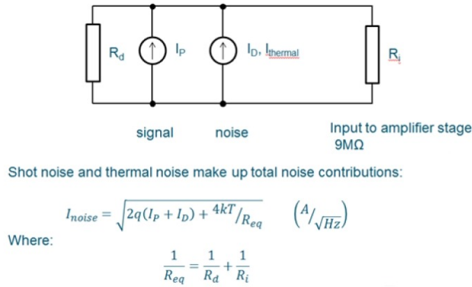
Figure 10: SPS sensors noise model electrical circuit ( R_d \sim 7 \text{ G}\Omega ).
