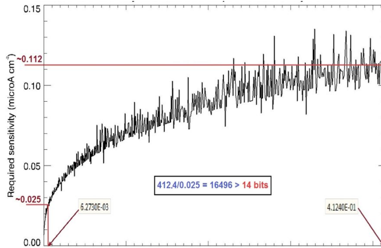
Figure 5: Required absolute ( \mu\text{A}/\text{cm}^2 ) longitudinal sensitivity and dynamic range as a function of the expected currents along the requirement box for a minimum displacement of 1 mm (the minimum is found at the edge of the requirement box, i.e. @ X = +100 mm, ref. to Table 1). The noise on the curve has a numerical computation origin.
