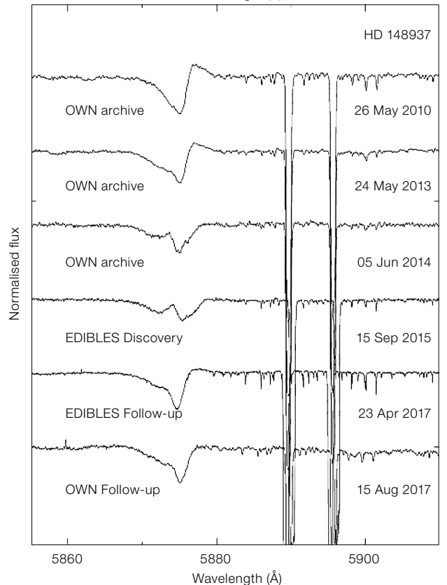
Figure 6. Upper Right: Archival observations showing the line profiles of the He I line at 5876 Å in HD 148937 between 1995 and 2010. Right: Archive observations from the Southern Galactic O- and WN-type stars (OWN) campaign (Barba et al., 2010) and EDIBLES observations of the same line between 2010 and 2017. Note how the character of the line profile changed markedly in 2014–2015 (Figure from Wade et al., in preparation).
