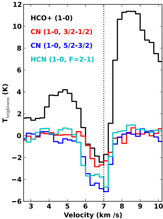
Figure 5. Continuum-subtracted spectra with an angular resolution of 1''.1 from the indicated transitions toward the HL Tau continuum peak. The adopted LSRK systemic velocity of 7 \text{ km s}^{-1} is indicated by the vertical dotted line. For comparison, the 2.9 mm peak continuum surface brightness at 1''.1 resolution is 5.75 \pm 0.01 \text{ K} .
