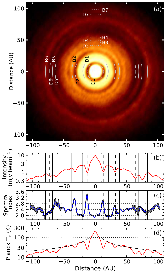
Figure 3. Panel (a) shows the deprojected 1.0 mm B6+B7 image of HL Tau (see Section 3.1.3); the angular resolution is 38.6 \times 19.3 mas (P.A. -20^\circ \pm 7^\circ ). Rings for which a full range of ellipse parameters could be fit are labeled horizontally (solid and dashed lines), while the less distinct rings are labeled vertically (dotted lines). Panels (b) and (c) show cross-cuts at P.A. = 138^\circ through the continuum peak of the 1.0 mm continuum and spectral index images shown in Figures 2(e) and (f) (positive values of distance correspond to the SE portion of Figure 2(e)). In panel (c) the gray region delineates the statistical 1\sigma spectral index uncertainty; it does not account for the absolute flux uncertainty. For the fully fitted rings, panels (b) and (c) show dashed lines for the locations of dark rings and solid lines for bright rings. The fitted offsets from the continuum peak (Table 2) have been taken into account. Panel (d) shows the same cross-cut as panel (b) but on a Planck brightness temperature ( T_B ) scale. Panels (b) and (d) are shown on a log scale on the y-axis. The dashed curve on panel (d) shows a representative power law for T_B as a function of radius with an exponent of -0.65 extending from the B1 peak; it is not a fit.
