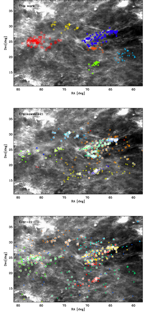
Fig. C.1. YSOs associated with Taurus-Auriga selected in this work (upper panel), Krolikowski et al. (2021) (middle panel), and Kerr et al. (2021) (lower panel). Colours and symbols indicate the sub-structures we found with DBSCAN, those derived by the Gaussian mixture model (GMM) in Krolikowski et al. (2021) , and those derived as EOM by Kerr et al. (2021) . White boxes in the middle and lower panels indicate the YSOs in common with our catalogue. YSOs are overplotted on an IRIS 100 \mu m image ( Miville-Deschênes & Lagache 2005 ).
