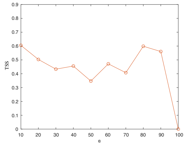
Fig. 3. Performance of forecasting models trained on magnetograms with different spatial resolutions. Original images are downgraded 1/\alpha times.
