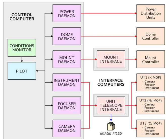
Fig. 16. Proposed control software architecture for a SAMNet sentinel.
