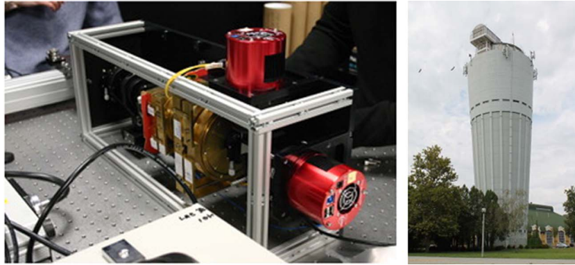
Fig. 13. A new design of the scaled-down SAMM (left panel) with the refurbished SAMNet HQ, Gyula Bay Zoltán Solar Observatory (GSO) (right panel).
