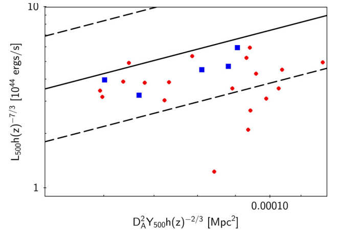
Figure 9. Distribution in the Y_{500}-L_{500} plane of the 24 missing ME-MACS clusters, compared with the best-fitting scaling relation (black continuous line) and its dispersion ( \pm 2\sigma , dashed lines) estimated in Planck Collaboration XXVII (2016). We mark with blue squares CC clusters and with red points NCC.
