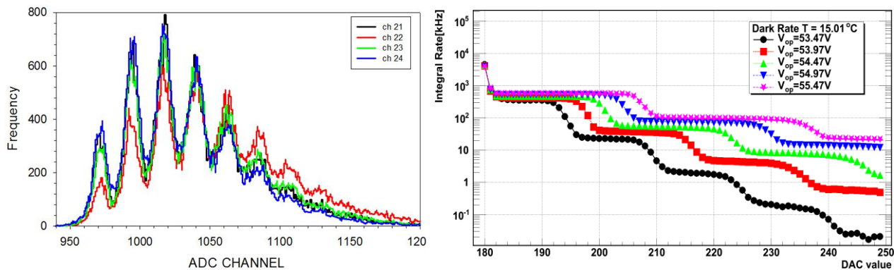
Figure 10. Left: Gain equalization of four camera pixels after the correction of the SiPM bias voltage obtained adjusting the input DAC voltages. Right: Staircase plots taken at different gain. The inflection points separate the count rates due to n -photoelectrons to n+1 -photoelectrons. The leftmost step shows the count rate due to a single photoelectron, the next one shows the count rate due to two coincident photoelectrons etc. The distance between the steps corresponds to the SiPM gain and it increases as the bias voltage raises.
