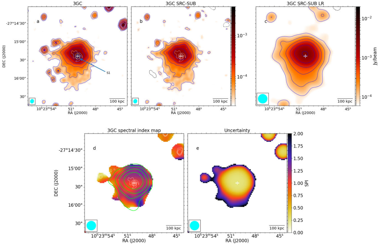
Figure 2. ACO 3444 3GC mini-halo. (a) Beam size ( 6''.8, 5''.9, -16''.0 ), local rms 1\sigma = 8.5 \mu\text{Jy beam}^{-1} , S1 marks the BCG, blue crosses indicate individual sources that were manually masked at HR; (b) SRC-SUB image, beam size, and colour-scale same as (a), local rms 1\sigma = 9.3 \mu\text{Jy beam}^{-1} ; (c) SRC-SUB 15'' LR image, local rms 1\sigma = 27.8 \mu\text{Jy beam}^{-1} ; (d) unsubtracted spectral index map; and (e) uncertainty map. The beam is shown in cyan in the bottom left corner of the images. Blue contours start at 3\sigma and increase by a factor of 2. Dashed black contours show the 3\sigma level. White contours show the emission from the HR image, which has beam size ( 3''.9, 3''.2, -9''.6 ) and local rms 1\sigma = 20.9 \mu\text{Jy beam}^{-1} . Green contours in (d) show the surface brightness of the SRC-SUB mid-band image and start at 5\sigma and increase by a factor of 2, where 1\sigma = 34.6 \mu\text{Jy beam}^{-1} . The white plus indicates the BCG position.
