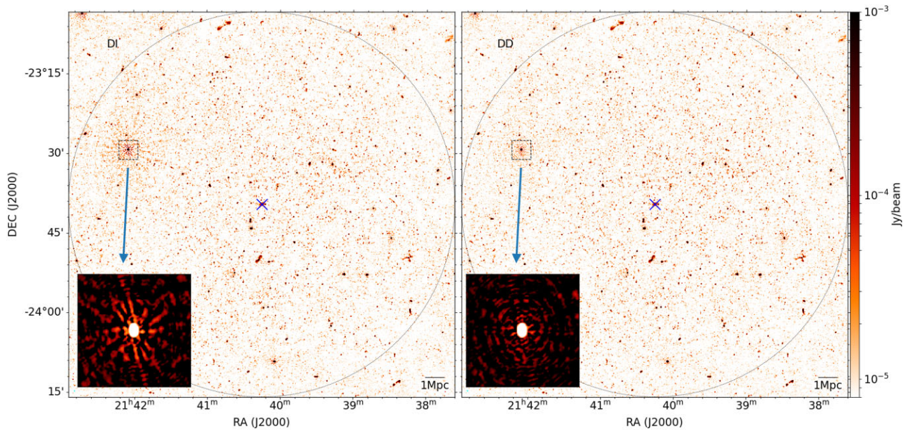
Figure D4. MACS J2140.2-2339 2GC versus 3GC artefacts. Left: 2GC image, beam size ( 7''.9 , 6''.3 , -9''.7 ), global apparent rms 7.2 \mu\text{Jy beam}^{-1} . Right: 3GC image, beam ( 7''.8 , 6''.2 , -8''.6 ), global rms noise 7.1 \mu\text{Jy beam}^{-1} . A blue cross marks the phase centre of the images. The thin-dashed black arc indicates the primary beam of the telescope. The bold-dashed black rectangle marks a bright point source with an arrow pointing to a zoomed inset of this source displayed in the inverse colourbar. The local rms decreased by just under a factor of two.
