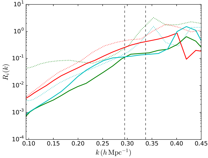
Figure 6. Ratios of Stokes Q (solid green), U (solid red), and V (solid cyan) vs. I power spectra averaged over a 0.092 < k_{\perp} < 0.097 \, h \, \text{Mpc}^{-1} region, whose center corresponds to a 175 m baseline. The dotted lines represent the corresponding power spectrum ratios from Figure 7 in Kohn et al. (2016). The left and right vertical dashed lines mark the horizon limit and 50 ns beyond it, respectively.
