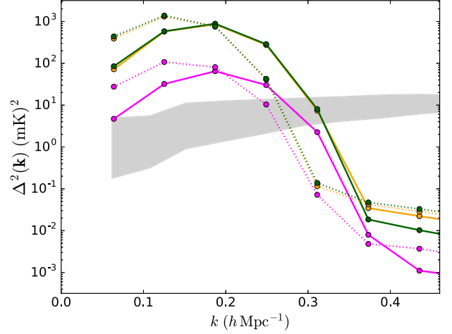
Figure 8. Left panel: polarized power spectra P_{Q,U} (orange and green lines respectively) for a 30 m baseline and an 8 MHz bandwidth centered at 150 MHz ( z = 8.5 ) from the diffuse polarized foreground D12 (solid) and D6 (dotted). The magenta line represents the leaked power spectra P_l . Right panel: same as the left panel but for \Delta_{Q,U}^2(k) . The shaded gray region represents power spectra of the 21 cm fiducial model from Lidz et al. (2008), with HI neutral fractions ranging between 0.21 and 0.82.
