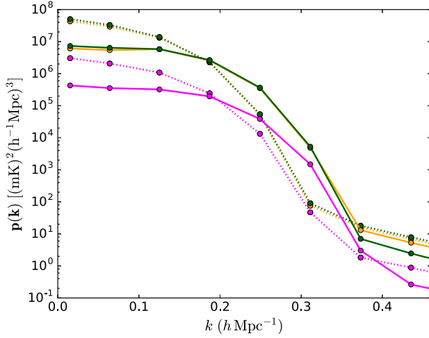
Figure 8. Left panel: polarized power spectra P_{Q,U} (orange and green lines respectively) for a 30 m baseline and an 8 MHz bandwidth centered at 150 MHz ( z = 8.5 ) from the diffuse polarized foreground D12 (solid) and D6 (dotted). The magenta line represents the leaked power spectra P_l . Right panel: same as the left panel but for \Delta_{Q,U}^2(k) . The shaded gray region represents power spectra of the 21 cm fiducial model from Lidz et al. (2008), with HI neutral fractions ranging between 0.21 and 0.82.
