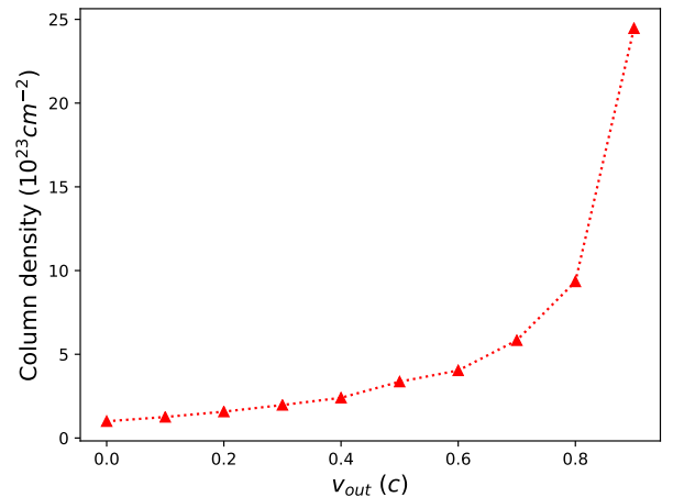
Fig. 3. Absorbing gas N_{\text{H}} required to reach a given value of the optical depth as a function of v_{\text{out}} . Spectral parameters are as in Fig. 2.
