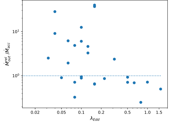
Fig. 5. Ratio of the relativistic-corrected outflow mass rate \dot{M}_{\text{out}}^{\text{rel}} to the inflow mass rate \dot{M}_{\text{acc}} , as a function of \lambda_{\text{Edd}} \equiv L_{\text{bol}}/L_{\text{Edd}} . The sample is as in Fig. 4. The dotted line corresponds to \frac{\dot{M}_{\text{out}}^{\text{rel}}}{\dot{M}_{\text{acc}}} = 1 .
