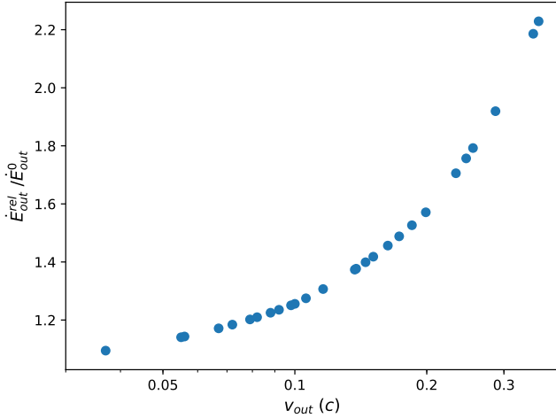
Fig. 4. Ratio of the relativistic-corrected energy transfer rates \dot{E}_{\text{out}}^{\text{rel}} to the original values \dot{E}_{\text{out}}^0 as a function of v_{\text{out}} , for a sample of ultra-fast outflows observed in AGNs (see Sect. 4 for details).
