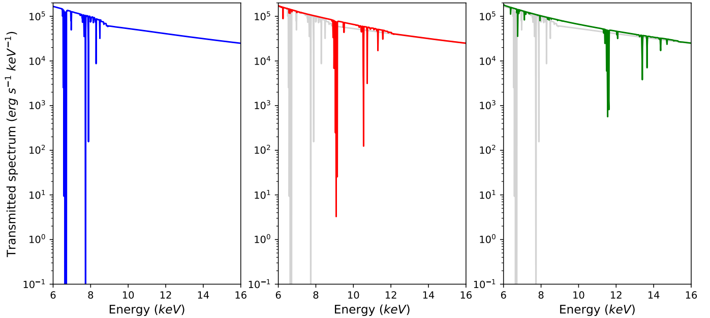
Fig. 2. Absorption spectra for increasing outflow velocity: v_{\text{out}} = 0.00 (left panel), = 0.30 (centre panel), = 0.50c (right panel). For comparison, in the centre and right panels we show the absorption spectrum for v_{\text{out}} = 0.00c (in light grey). See Sect. 3 for details on the spectral parameters used in this simulation.
