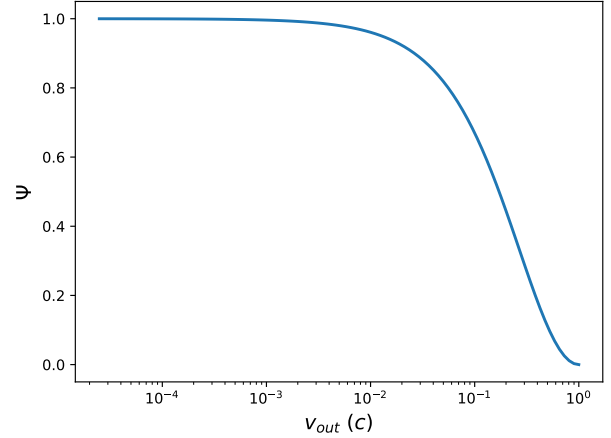
Fig. 1. Deboosting factor \Psi in the gas reference frame K' as a function of v_{\text{out}} assuming \theta = 180^\circ . For speeds lower than 0.1c , the radiation intercepted by the outflow and by the (rest-frame) observer at infinity are virtually the same. For higher speeds, the fraction of intercepted radiation drops dramatically due to special relativistic effects.
