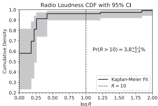
Figure 4. The cumulative density function F(R) of the radio-loudness parameter R as fit by the Kaplan–Meier estimator. The shaded region represents a 95 percent confidence interval and the vertical dashed line indicates the radio-loud threshold at R = 10 . The radio-loud fraction is estimated as \Pr(R > 10) = 1 - F(R = 10) = 3.8^{+6.2}_{-2.4} per cent.
