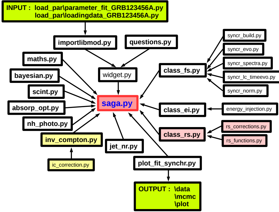
Figure 2: Structure of SAGA. Yellow boxes indicate the sections nearing completion; red boxes indicate the incomplete parts. Input/Output are labeled in green.
