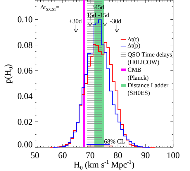
Figure 2. Marginalized probability distribution functions of H_0 . The results of the flat \Lambda CDM models listed in Table 1 are shown by the red and blue histograms (on the bottom, the corresponding 68% CL intervals). The vertical arrows show the inferred median values of H_0 (in the (p) case) if the time delay of SX differs from 345 days by 15 or 30 days. Credible intervals, at 1\sigma CL, from H0LiCOW (Bonvin et al. 2017), Planck (Planck Collaboration XIII 2016) and SH0ES (Riess et al. 2016) are indicated in gray, magenta and green, respectively.
