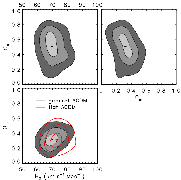
Figure 3. Constraints on the cosmological parameters. The model \Delta t(p) (see Table 1) in flat (red) and general (gray) \Lambda CDM models with uniform priors on the values of the cosmological parameters ( H_0 \in [20, 120] km s -1 Mpc -1 , \Omega_m \in [0, 1] and \Omega_\Lambda \in [0, 1] ) is shown here. The cross symbols and the contour levels on the planes represent, respectively, the median values and the 1\sigma , 2\sigma , and 3\sigma confidence regions, as obtained from MCMC analyses.
