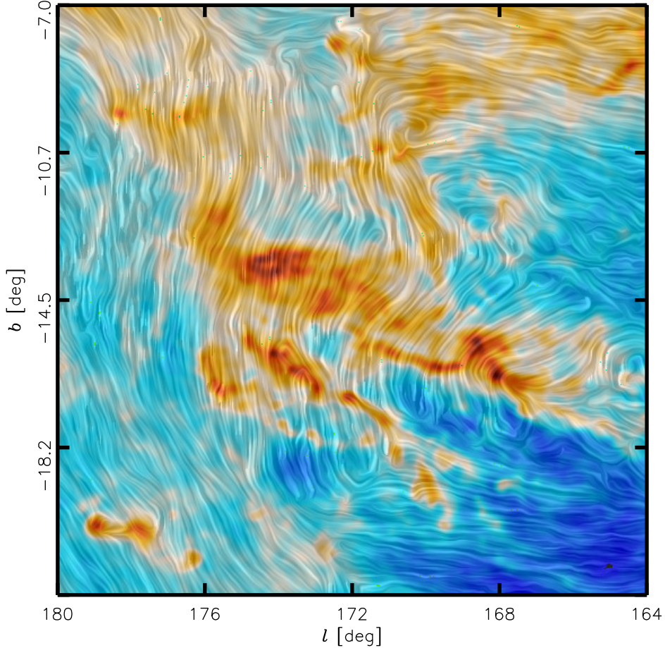
Fig. 1. Magnetic field and column density measured by Planck towards the Taurus MC. The colours represent column density. The “drapery” pattern, produced using the line integral convolution method (LIC, Cabral & Leedom 1993), indicates the orientation of magnetic field lines, orthogonal to the orientation of the submillimetre polarization.
