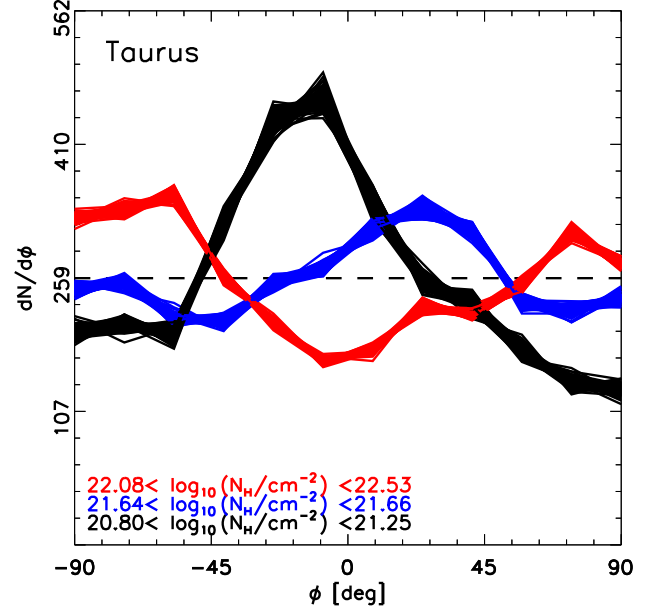
Fig. B.1. HROs in the Taurus region that correspond to the indicated N_{\text{H}} bins. The plotted values are obtained using the original \tau_{353} map at 10' resolution and maps of the Stokes parameters Q_r and U_r , which correspond to 1000 random noise realizations. Each realization is generated using a Gaussian probability density function centred on the measured values Q and U with variances \sigma_Q^2 and \sigma_U^2 .
