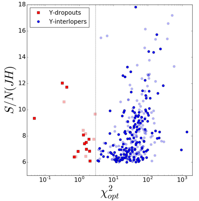
Figure 5. Comparison between the S/N( JH_{\text{det}} ) and the optical \chi^2 for Y_{105} -dropouts for the GSd field. Colors and symbols are as in Figure 1. The dotted vertical line indicates the separation between interlopers and dropouts adopted in this work.
