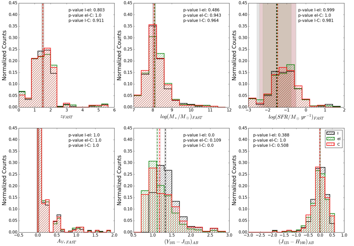
Figure 11. Distribution of redshifts, stellar masses, star-formation rates, dust extinctions, and colors for Y-interlopers in the original sample (“I,” black lines), Y-interlopers in the enlarged sample (“el,” green lines), and for interlopers appearing as contaminants after the MC experiment (“C,” red lines). Stellar population properties have been estimated from the photometry with FAST (Kriek et al. 2009). Values indicated are the probabilities that two distributions are drawn from the same parent distribution, according to the Kolmogorov–Smirnov test.
