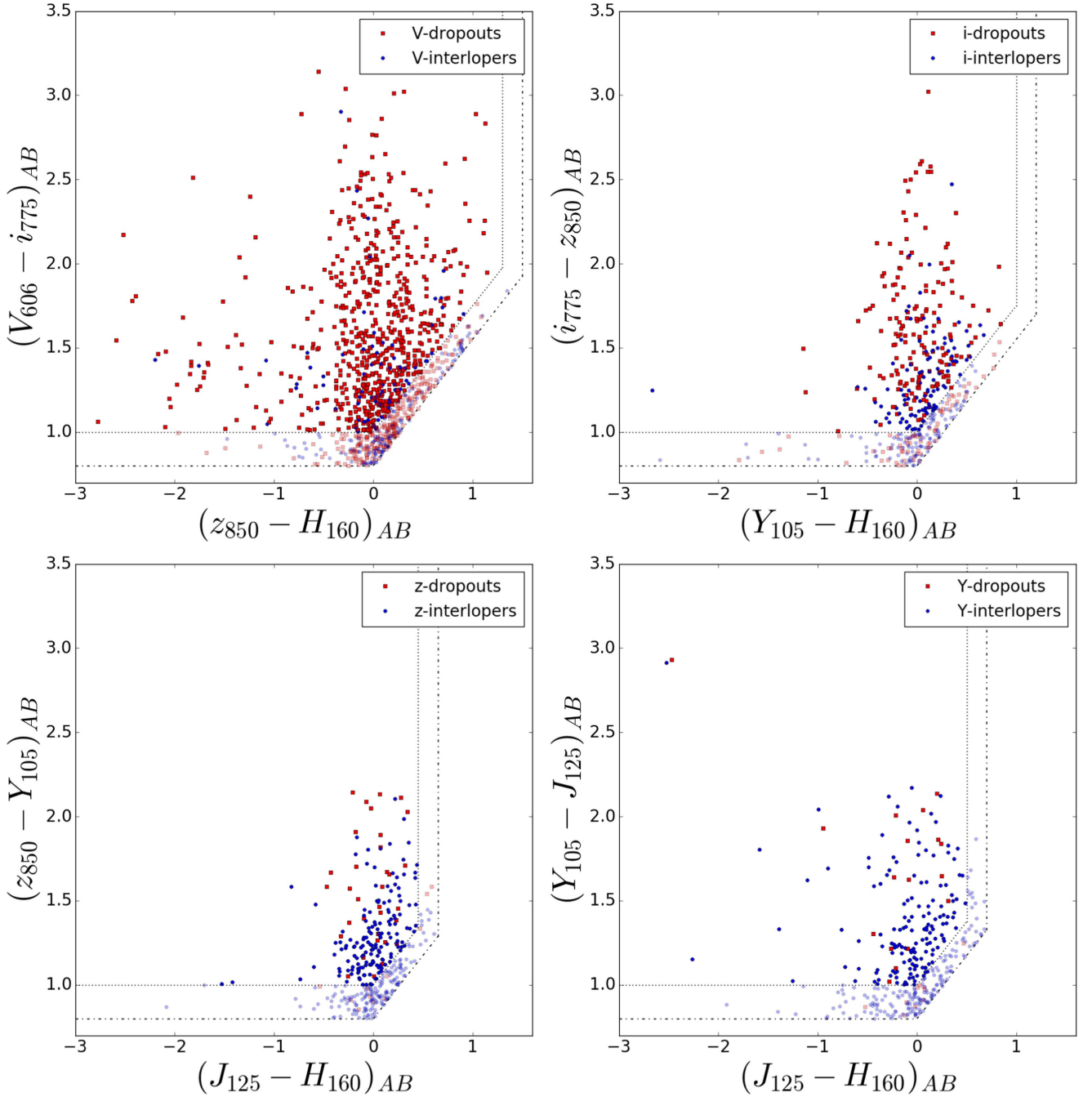
Figure 1. Color–color selection box used to identify V_{606} –(upper left), i_{775} –(upper right), z_{850} –(bottom left) and Y_{105} –dropouts (bottom right) over the GSd field. Red squares represent dropouts, i.e., high- z sources with no flux blueward of the Lyman-break; blue circles represent interlopers, i.e., high- z candidates showing a detection in the blue bands. Dashed lines represent the boundaries of the original sample selection; dashed–dotted lines represent the boundaries of the enlarged sample (see the text for details). Darker symbols refer to the original selection, lighter ones refer to the enlarged selection.
