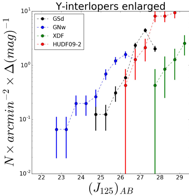
Figure 6. Surface density distribution of Y_{105} -interlopers in the enlarged samples for all the fields considered in this study, as indicated in the labels. Each sample is plotted down to its formal 5\sigma magnitude limit (from Bouwens et al. 2015). The best power-law fit of the sample is \log(N/\text{arcmin}^2/\Delta(\text{mag})) = (0.35 \pm 0.1) \times J_{125} + (-9.0 \pm 0.4) .
