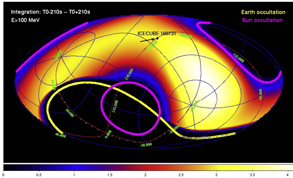
Figure 1. Hammer–Aitoff projection, in Galactic coordinates, of the AGILE gamma-ray exposure in ( \text{cm}^2 \text{ sr} ) (bin size of 0.5^\circ ) after one complete rotation in spinning mode, time-centered at the ICECUBE-160731 event time T_0 . The neutrino event error circle is shown in black. The magenta and yellow contours show, respectively, the Sun/anti-Sun exclusion regions and the average Earth occultation during the considered integration time: ( T_0 - 210 ; T_0 + 210 ) s.
