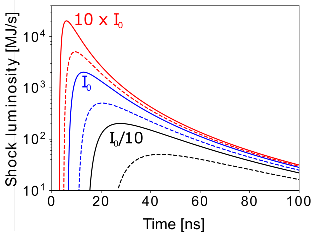
FIG. 7. Shock luminosity for three different laser intensities (colors) computed at z = 1.2 cm from the 1D self-similar model described in the main text. Full line: \lambda = 1.06 \mu\text{m} ; dashed line: \lambda = 0.53 \mu\text{m} . The stream radius is taken to be 0.1 cm.
