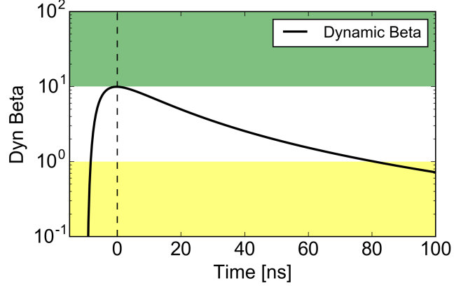
FIG. 5. Same as Fig. 4 for \beta_{dyn} = \frac{\rho_{stream}v_{stream}^2}{B^2/2\mu_0} , calculated for B = 2 \times 10^5 \text{ G} (20 T). The green area represents the region \beta_{dyn} > 10 , and the yellow area represents the region \beta_{dyn} < 1 -keeping the color label of Fig. 3. Note that an other interesting information, the ram pressure \rho_{stream}v_{stream}^2 , is directly readable on that plot by multiplying the \beta_{dyn} by the magnetic pressure B^2/2\mu_0 = 160 \text{ MPa} . N.B. Regardless of slight fluctuations it can have within the jet [13], the initial strength of the magnetic field is the pertinent one in order to characterize the \beta_{dyn} , as being the field effectively encountered by the flow at the impact with the obstacle.
