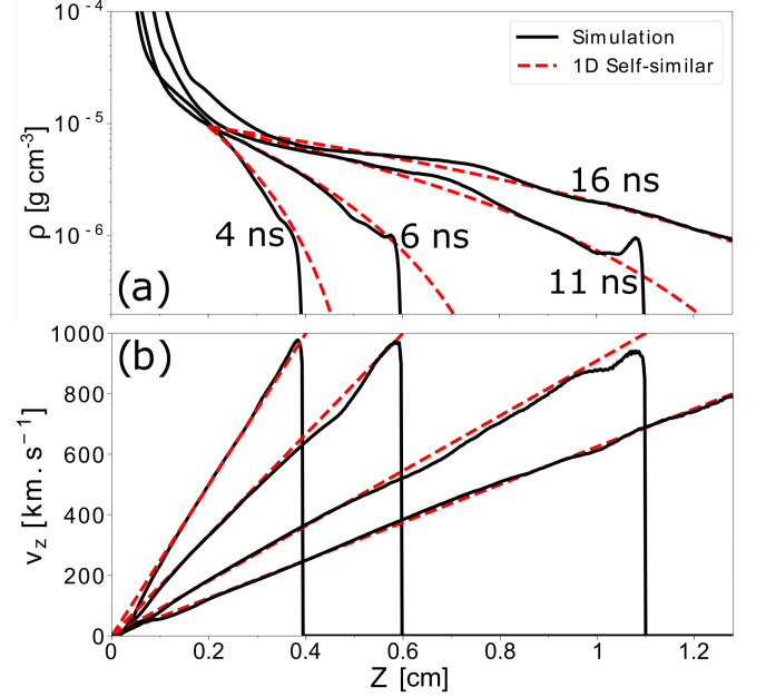
FIG. 2. GORGON longitudinal density profiles (top) and velocity (bottom) compared to a 1D self-similar analytical model (see text), at different times after the start of the expansion (at t = 0 ). The profiles are made via an average around the z -axis over a radius of 7 \times 10^{-2} cm, i.e. the laser focal spot.
