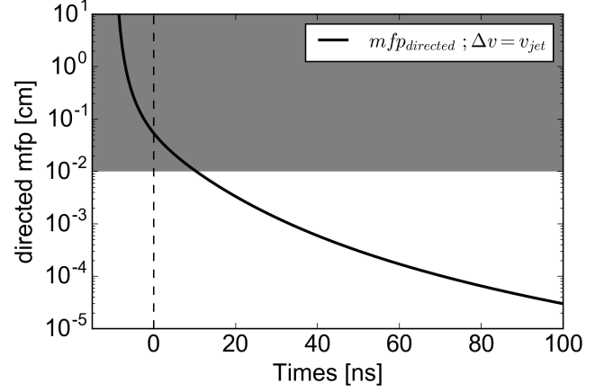
FIG. 4. Directed mean free path as a function of time, at the obstacle location, i.e. \sim 1.2 \text{ cm} from the stream target, following the 1D self-similar model. The gray area displays the transition region for which mfp_{dir} = L/10 = 10^{-2} \text{ cm} , where the shock front size over which the particle are stopped becomes sufficiently small compared to the characteristic size of the system L , i.e. the stream radius (see also discussion linked to Fig. 3). The time in the abscissa takes its origin at the 750 \text{ km s}^{-1} plasma component arrival time, as also highlighted by the vertical dashed line.
