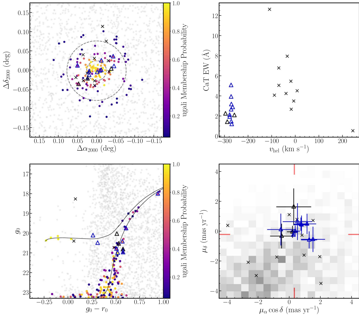
Figure 2. (Top left) Spatial distribution of stars within a small region (radius of \sim 0^\circ 25 ) centered on Pegasus IV. Stars with u_{\text{gali}} probability p_{\text{ugali}} > 0.05 are colored by their membership probability, while stars with p_{\text{ugali}} < 0.05 are colored in gray. Blue triangles denote the nine clear candidate spectroscopic members, while black triangles denote candidate spectroscopic members with uncertain status. Black crosses denote stars observed spectroscopically but deemed nonmembers. Contours representing 1\sigma and 3\sigma are overplotted with a gray dashed line, assuming \epsilon = 0 (given the upper limit reported in Table 1). (Top right) calcium triplet equivalent width (CaT EW, in angstroms) vs. heliocentric radial velocity ( v_{\text{hel}} , in kilometers per second) for all 23 stars observed with IMACS at S/N > 3 . (Bottom left) Color-magnitude diagram for the same region shown in the top left panel, with the same color/symbol scheme as the preceding panels. The two candidate HB variable stars are seen as blue triangles at g_0 - r_0 \sim 0.25 . One member lacking DECam photometry is excluded here. The majority of nonmembers (especially those selected based on Gaia alone) have redder colors than the axis range shown here. (Bottom right) Gaia proper motions of the stars observed spectroscopically with IMACS, overlaid over a 2D proper motion histogram of all Gaia sources within a radius of \sim 0^\circ 25 . The candidate spectroscopic members cluster closely near the systemic mean proper motion of (\mu_{\alpha*}, \mu_\delta) = (0.33, -0.22) mas yr -1 , denoted by the red hatch marks (see Section 4.7).
