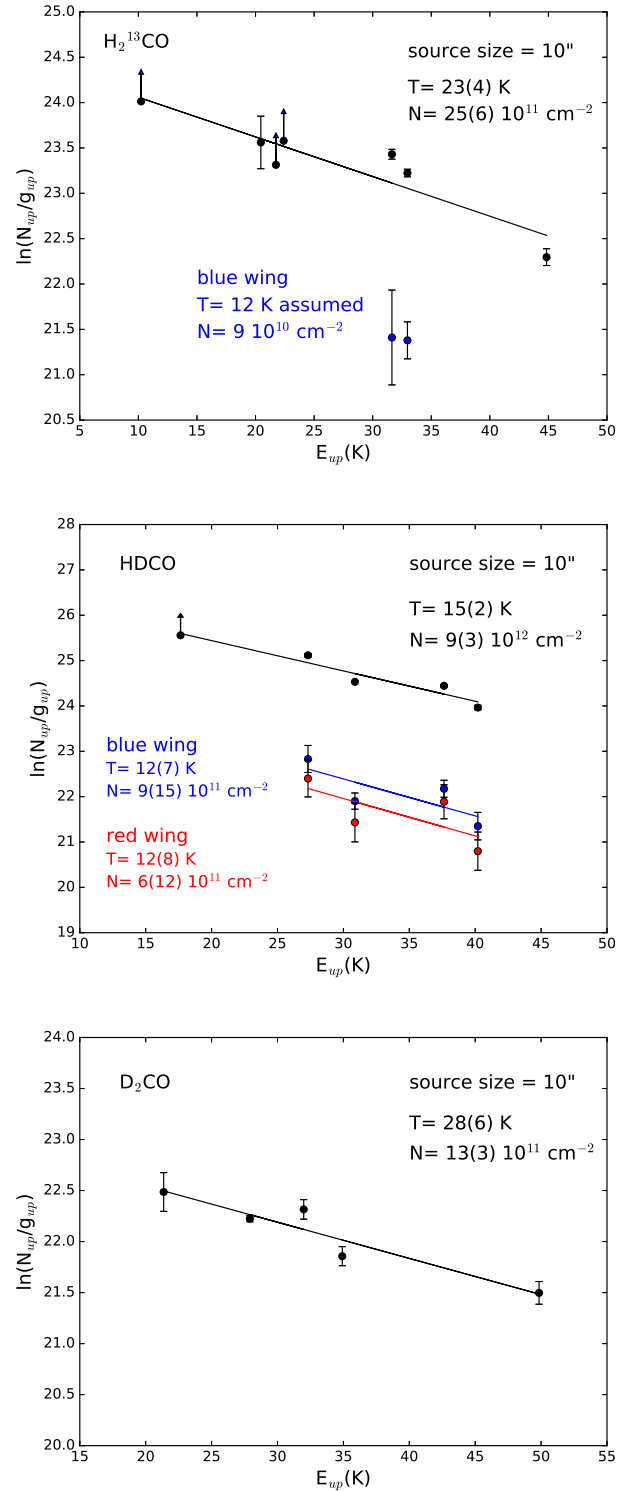
Figure 6. Rotation diagrams for \text{H}_2^{13}\text{CO} (upper panel), HDCO (middle panel) and \text{D}_2\text{CO} (lower panel). An emitting region size of 10'' is assumed (see text). The parameters N_{\text{u}} , g_{\text{u}} , and E_{\text{up}} are, respectively, the column density, the degeneracy and the energy (with respect to the ground state of each symmetry) of the upper level. The derived values of the rotational temperature are reported. Arrows are for the lines affected by wobbler contamination (see Section 3.2) and thus considered as lower limits.
