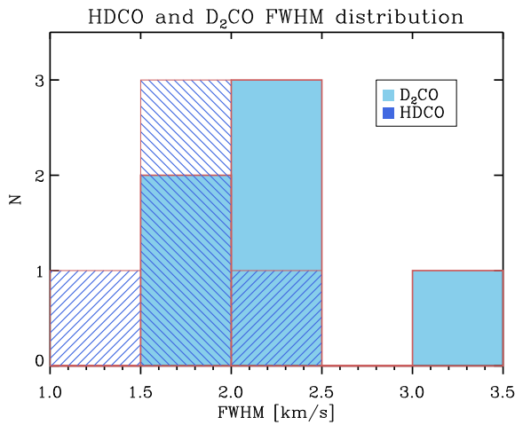
Figure 2. Distribution of the linewidth (FWHM) of the observed HDCO and D 2 CO lines. Cyan is for D 2 CO and blue hatched is for HDCO.
