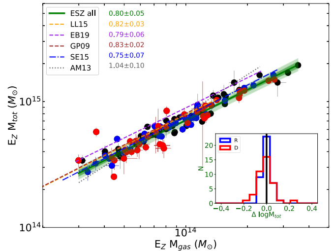
Figure 5. M_{\text{tot}} – M_{\text{gas}} relation for the ESZ clusters investigated in this work. The most relaxed and most disturbed clusters are shown in blue and red, respectively. The green line represents the fitted relation with \gamma free to vary in the fit. The dark and light shaded areas represent the 1\sigma statistical error and scatter, respectively. All the relations are plotted only in the mass range covered by the individual study. In the inset plot, we show the histogram of the log space residuals from the fitted M_{\text{tot}} – M_{\text{gas}} relation. The agreement between the slopes obtained with samples having a different fraction of relaxed and disturbed systems and between the subsamples of relaxed and disturbed clusters in the ESZ sample suggests that this relation is insensitive to the dynamical state of the clusters. However, the offset observed in the normalization may suggest that the mass range of the investigated samples plays a role because of the increasing gas fraction for high-mass systems. The acronyms in the legend are described in Sections 5.1, 5.4, and 5.6.
