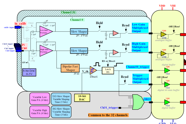
Figure 9: Block diagram of the EASIROC chip [9]
