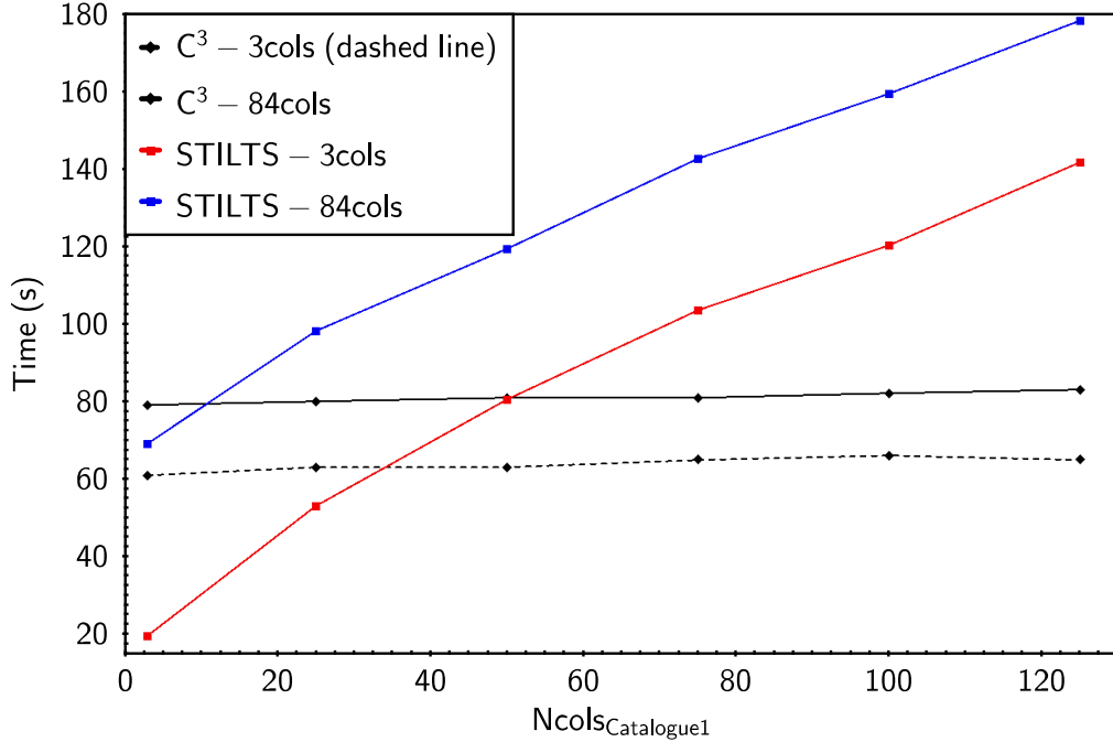
Figure 8. Computational time as function of the number of columns of the first input catalog for the C^3 cross-matching phase and STILTS, considering a second catalog with 3 (black dashed line for C^3 , red or light gray line for STILTS) and 84 (black line for C^3 and blue or dark gray for STILTS) columns.
