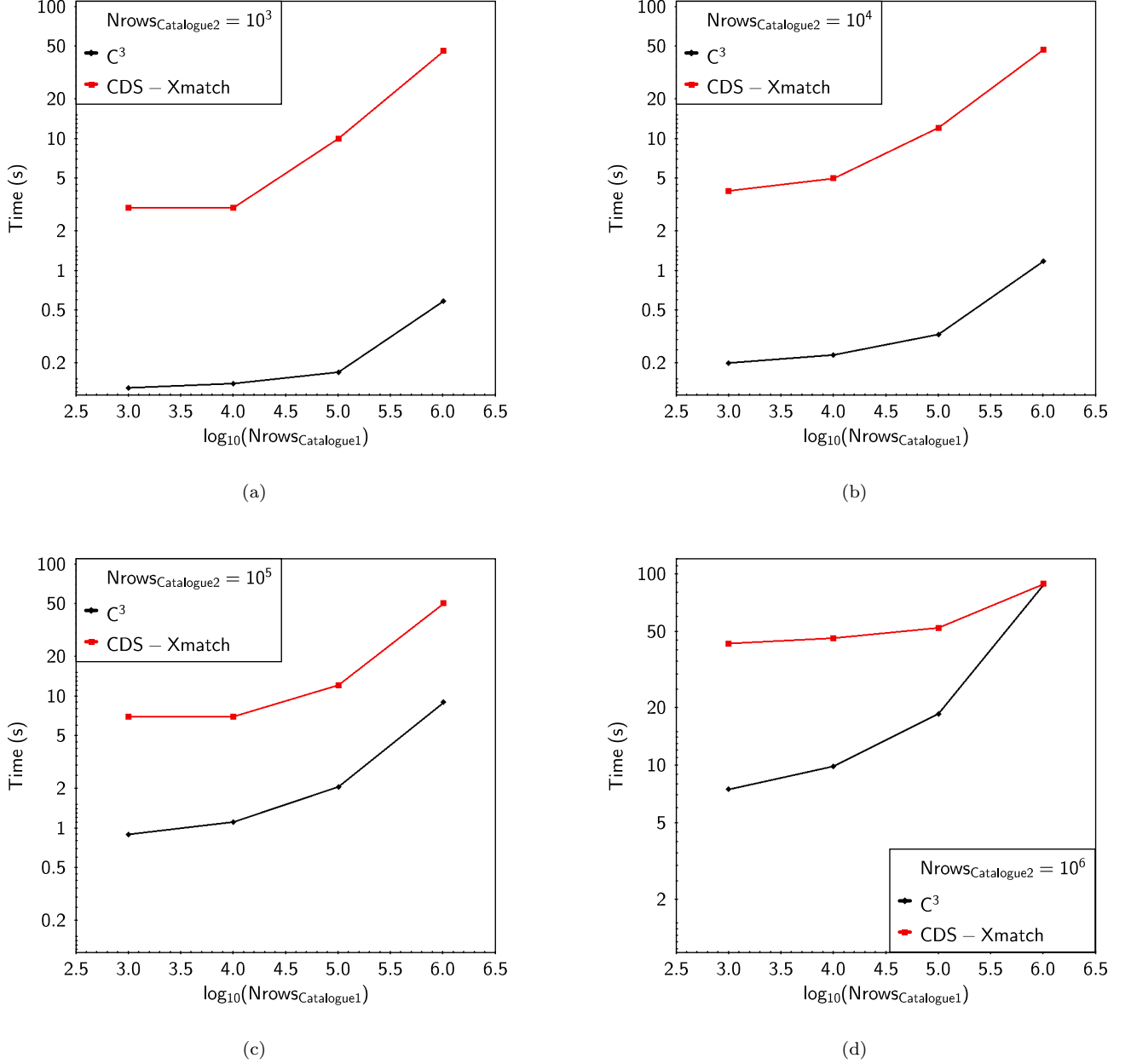
Figure 9. Computational time as function of the number of rows of the first input catalog for the C^3 cross-matching phase (black) and CDS-Xmatch (red or gray) for four different dimensions of the second catalog: (a) 1000 rows, (b) 10,000 rows, (c) 100,000 rows, (d) 1,000,000 rows. Considering only the cross-matching step of CDS-Xmatch, its performance are better than C^3 .
