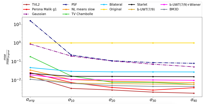
Fig. C.6. H160 depth variation comparison plot. On the x-axis the H160 images with Gaussian noise standard deviation equal to 1, 10, 20, 30 and 40 times the original value, whereas on the y-axis \frac{mse}{mse_{Original}} .
