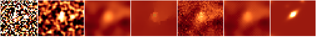
Fig. D.10. VIS crops visual comparison: Original, PSF, Perona-Malik, TVL2, Bilateral, TV Chambolle, Noiseless. The green boxes are the detected objects regions. The central object has been detected with a SNR of 26.74 with magnitude of 26.13
