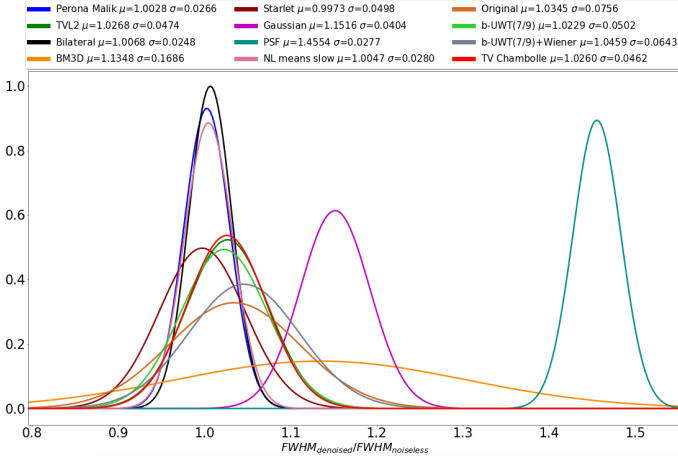
Fig. 5. Step 4: FWHM conservation test on stars. On the x -axis we plot the FWHM_{denised}/FWHM_{noiseless} , where FWHM_{noiseless} is the FWHM of the objects measured on the Noiseless image. \mu and \sigma are the mean and the standard deviation of the distribution of FWHM_{denised}/FWHM_{noiseless} .
