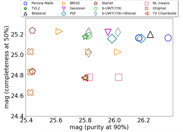
Fig. 13. Ground-based real Images Completeness & Purity (HAWK-I and HAWK-I UDS). On the x-axis the magnitude at which the purity drops below 90%, on the y-axis the magnitude at which the completeness drops below 50%. Each symbol is referred to a different denoising method, which can be present multiple times in the plot due to different combinations of detection parameters, see text for details. The positions of the symbols are slightly randomized to improve readability.
