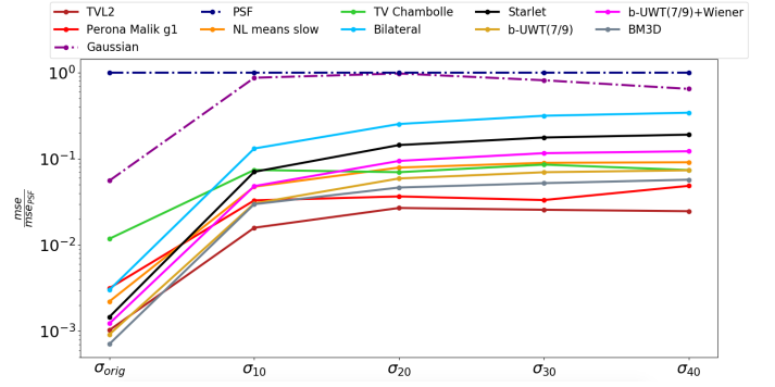
Fig. C.5. H160 depth variation comparison plot. On the x-axis the H160 images with Gaussian noise standard deviation equal to 1, 10, 20, 30 and 40 times the original value, whereas on the y-axis \frac{mse}{mse_{PSF}} .
