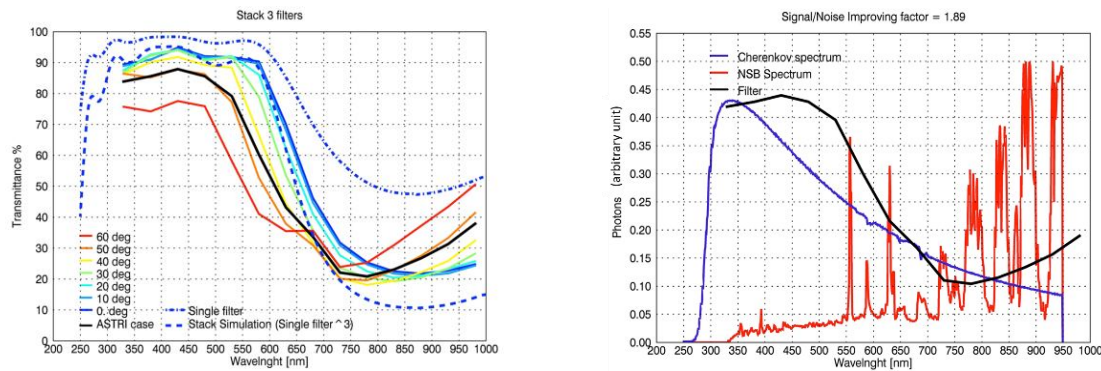
Figure 3: Spectrosil transmittance vs wavelength at photon incidence angles between 0^\circ and 60^\circ (left panel). The transmittance (averaged with respect to the incidence angle) of the filter window used in the ASTRI camera prototype (black curve) is superimposed to the Cherenkov and NSB spectrum (right panel) showing the drop off at wavelengths greater than 700 nm.
