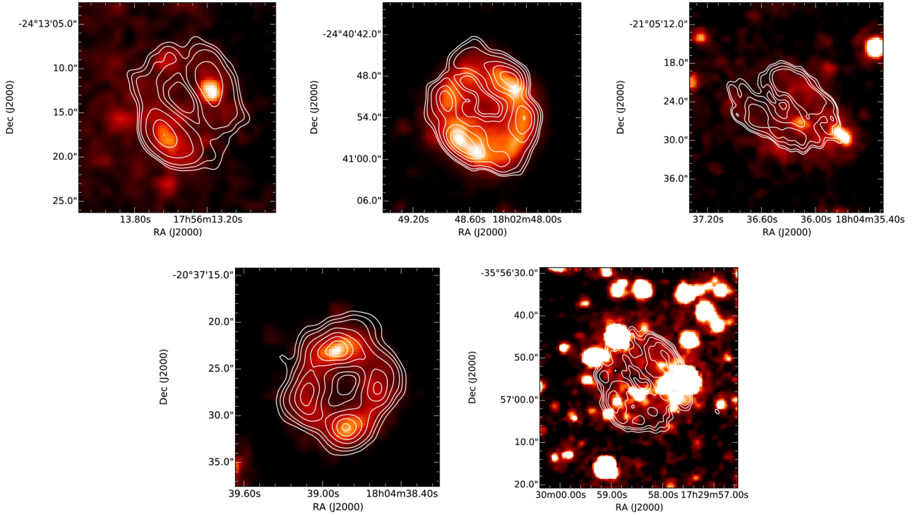
Figure 12. Superposition of IRAC 8- \mu m images and 6-cm contours of the ‘elliptical’ bubbles. From left to right: (row 1) MGE 005.2641+00.3775, MGE 005.6102–01.1516, MGE 008.9409+00.2532; (row 2) MGE 009.3523+00.4733, MGE 352.3117–00.9711 (for this last bubble, 4.5 \mu m image is used instead).
