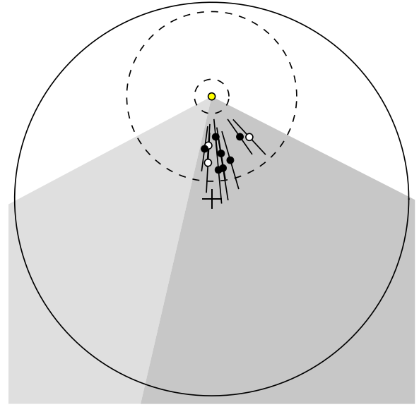
Figure 19. Calculated position of the elliptical bubbles (solid circles and error bars) and filled elliptical bubbles (open circles and error bars) on to the Galactic plane. The Sun is represented with a yellow circle, the Galactic Centre with a cross and the Galaxy outer limit is assumed to be 16 kpc from the centre (solid circumference). The entire shaded area represents the portion of the Galactic plane covered by MIPS GAL. Its darker part satisfies \delta > -40^\circ , the lower declination limit of VLA. The two dashed circumferences represent the distance from the Sun at which a nebula with a diameter of 0.4 pc is seen under an angle of 12 (outer circumference) and 60 arcsec (inner).
