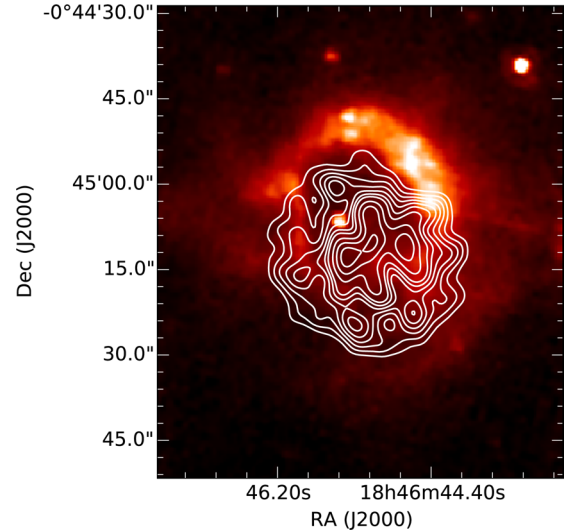
Figure 16. Superposition of 8- \mu m image and 6-cm contours of MGE 031.7290+00.6993.
