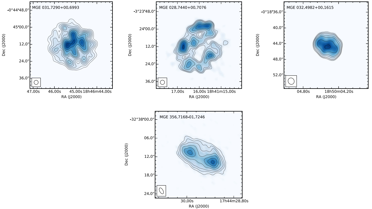
Figure 4. 6-cm images of the bubbles MGE 031.7290+00.6993, MGE 028.7440+00.7076 and MGE 032.4982+00.1615 (row 1, from left to right; morphology ‘O’ of Table 2); (row 2) MGE 356.7168–01.7246 (morphology ‘B’ of Table 2).
