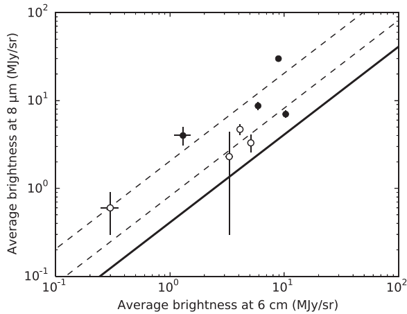
Figure 15. Average brightness at 8 \mu m against average brightness at 6 cm for the ‘elliptical’ bubbles (solid circles) and for the ‘filled elliptical’ bubbles (open circles). The solid line represent a pure free–free emission, while the two dotted lines represent a brightness respectively twice and five times greater.
