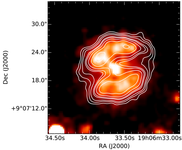
Figure 14. Superposition of 8- \mu m image and 6-cm contours of MGE 042.7665+00.8222.
