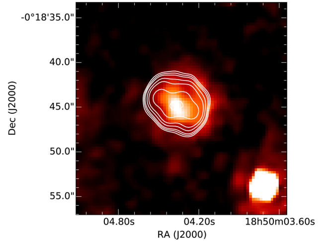
Figure 18. Superposition of 8- \mu m image and 6-cm contours of MGE 032.4982+00.1615.
