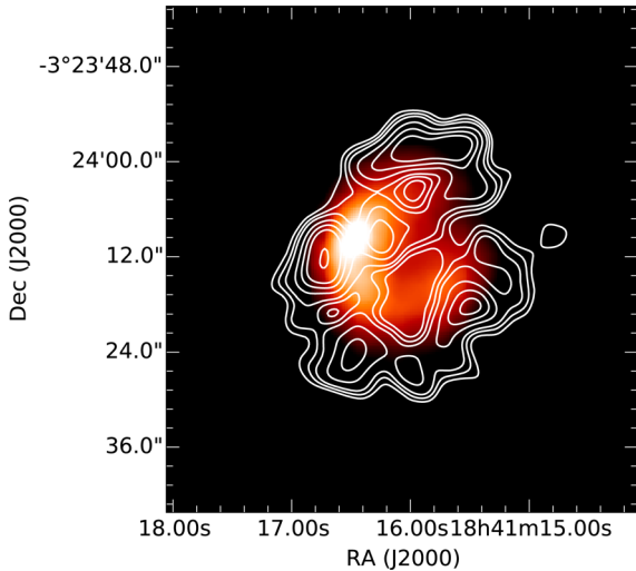
Figure 17. Superposition of 24- \mu m image and 6-cm contours of MGE 028.7440+00.7076.
