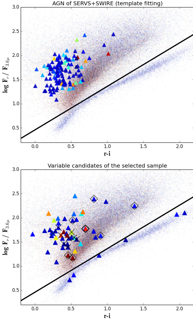
Fig. 5. Flux ( F_\lambda ) ratios between the r band and 3.6\ \mu versus r - i colour. In the top panel , the triangles represent sources flagged as AGN in the SERVS+SWIRE catalogue, on the basis of optical/IR template fitting (133 AGN, see Sect. 5.3.1). In the bottom panel the triangles represent the 57 sources belonging to our “selected sample” with available i , r , and 3.6\ \mu photometry in the SERVS+SWIRE catalogues (see Sect. 5.3.1). Diamonds and crosses label the SN and X-ray detected sources, respectively (see Sect. 5.2). In both panels, the small points represent the whole SERVS+SWIRE control sample with available r , i , 3.6\ \mu photometry (82254 sources). The colours from red (extended sources) to blue (pointlike sources) indicate the increasing stellarity (defined in footnote 9) as measured from the VST images for our “selected sample” or extracted from the SERVS+SWIRE catalogues in the optical r band for the control sample. The solid line divides the plane into the stellar region and the non-stellar region.
