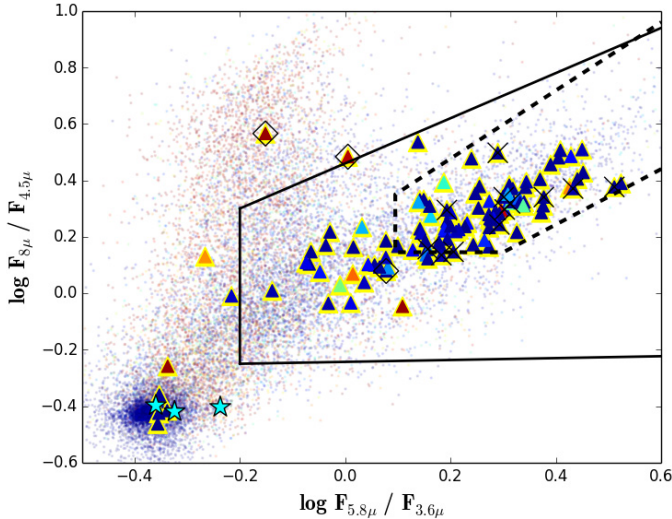
Fig. 6. Flux ( F_\lambda ) ratio (logarithmic) at 5.8 and 3.6\ \mu versus flux ratio at 8 and 4.5\ \mu . Small points: SERVS+SWIRE 18436 sources; triangles (enclosed in yellow edges): 115 sources in common with the selected sample (see Sect. 5.3.2). Cyan stars: stars; diamonds: SN. Crosses: X-ray detected sources. The colours of the triangles and of the small points from red (extended sources) to blue (pointlike sources) indicate the increasing stellarity (as in Fig. 5). The solid line is the Lacy et al. (2004) region and the dashed line the Donley et al. (2012) region.
