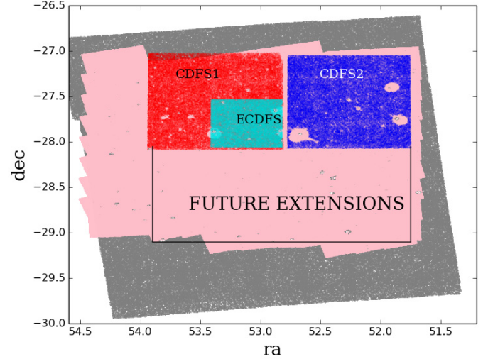
Fig. 1. Region covered by the VST observations compared to other overlapping surveys. Red: VST-CDFS1, blue: VST-CDFS2, grey: SWIRE, pink: SERVS, cyan: ECDFS area. The holes in the CDFS1 and CDFS2 are due to the masks we applied to exclude bright stars, spikes, and reflection features, as explained in detail in Sect. 3.
