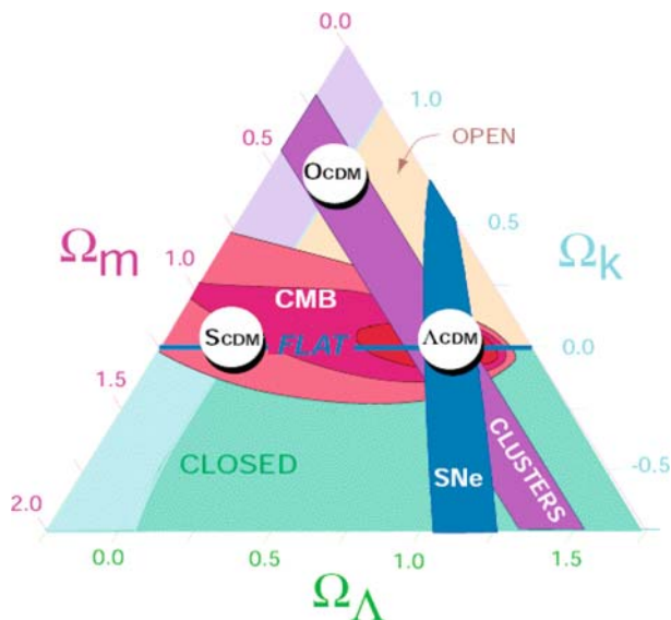
Fig. 5.16. The cosmic triangle [53], see http://www.phy.princeton.edu/~steinh/ . The complementarity of the three classic cosmological tests is clearly shown
