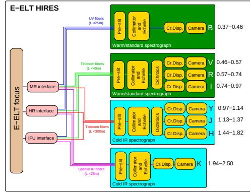
Fig. 1. Possible HIRES architecture with spectral separation in four spectrographs.
