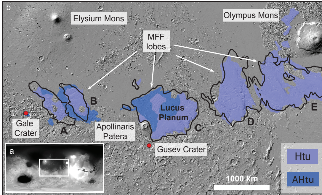
Figure 1. Geomorphologic and geologic setting for Lucas Planum: a) Location of the greater Medusa Fossae Formation (MFF) deposits, the sub-figure b is outlined in white. b) Extent of the Medusa Fossae Formation as outlined, in black, by Kerber et al. [2011]. The MFF lobes are also indicated with letters, according to Harrison et al. [2010]. Lucas Planum constitutes the centre lobe of the MFF. Units from the revised global geological map of Mars [ Tanaka et al. , 2014] are indicated Htu and AHtu . The location of the NASA MER Spirit rover landing Site in Gusev crater and NASA MSL Curiosity in Gale crater are indicated. Figure 1a is a global map in equirectangular projection, centred at longitude 180. Figure 1b is a map centred on Lucas Planum and covering the MFF, in equirectangular projection, and centred at 180° E. The longitudinal extension is about 5000 km. Latitude range is from -30^\circ to 30^\circ , longitude ranges from 130^\circ E to 230^\circ E.
