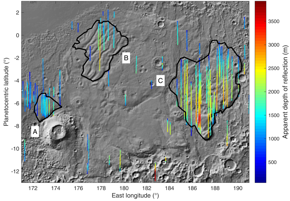
Figure 4. Map of the location and apparent depth of subsurface echoes in Lucas Planum. Apparent depth is coded according to the colour scale on the right, and differs from real depth by a factor \sqrt{\epsilon} (see Eq. 1). Black contours outline what appear to be different morphologic provinces within Lucas Planum.
