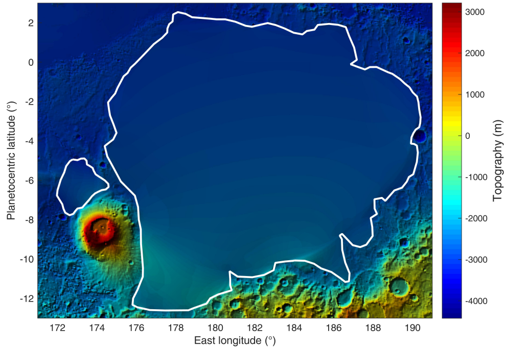
Figure 5. Topographic map of the Lucus Planum area, based on the MOLA dataset.
