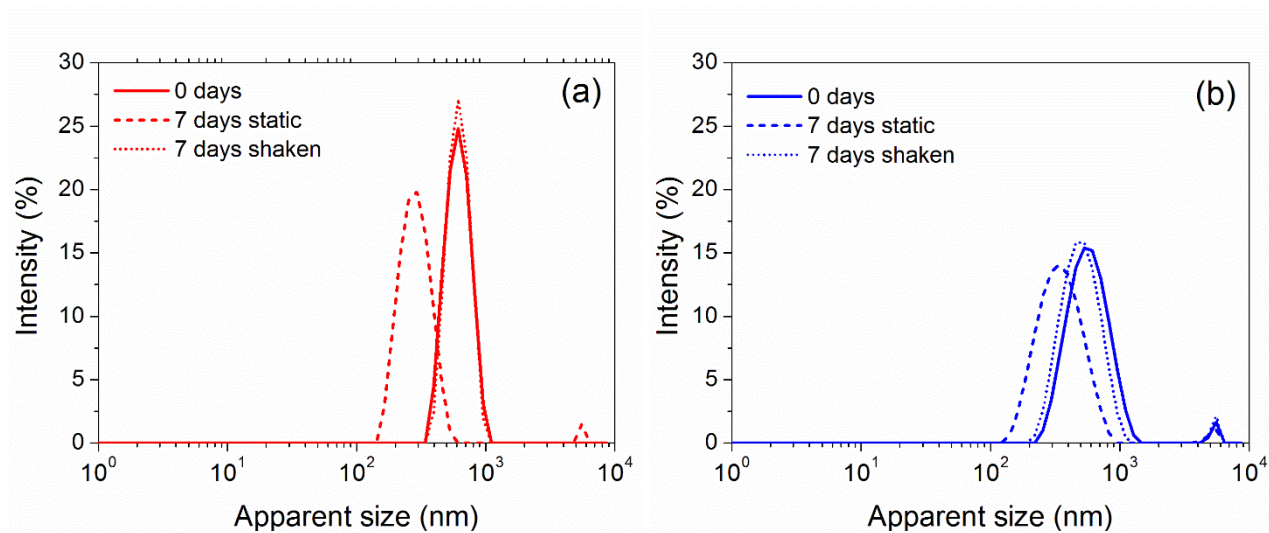
Figure 4: Apparent size distribution for 0.025 wt% samples: (a) S-GnP/water nanofluid and (b) P-GnP/water nanofluid.
