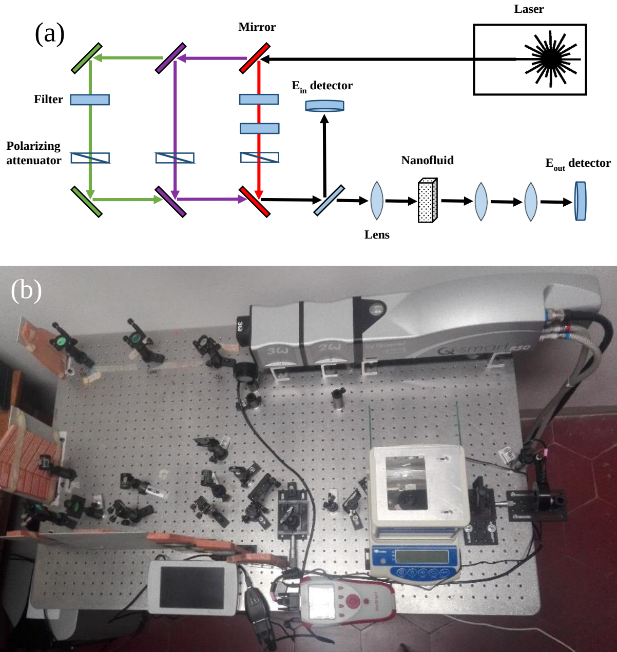
Figure 1: Scheme (a) and real image (b) of the laser experiment setup.
