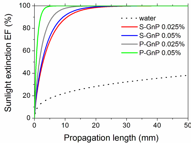
3 Figure 9: Calculated sunlight extinction as a function of the propagation length within the 4 nanofluids. 5
