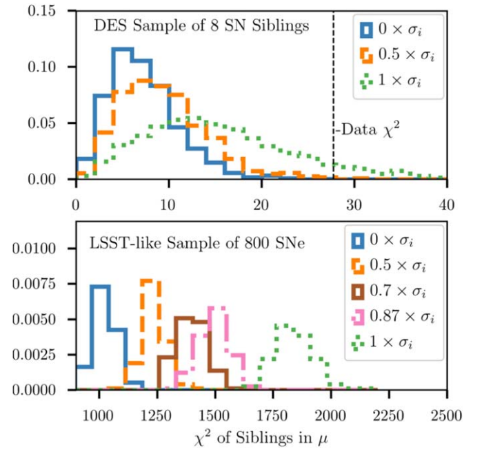
Figure 4. (Top) From evaluations of the distance modulus \mu , the predicted \chi^2_S distribution from simulations of eight DES SN siblings and the \chi^2_D from the real data set—as presented in Figure 3. The three histograms show distributions of \chi^2_S of 1000 samples of eight siblings from simulations with no intrinsic scatter (blue), half intrinsic scatter (red) and full intrinsic scatter (green). (Bottom) Again for \mu , the predicted \chi^2_S distribution from simulations of 800 pairs of LSST SN siblings. Similar to above, the multiple histograms are created for simulations with different scales of the intrinsic scatter.
