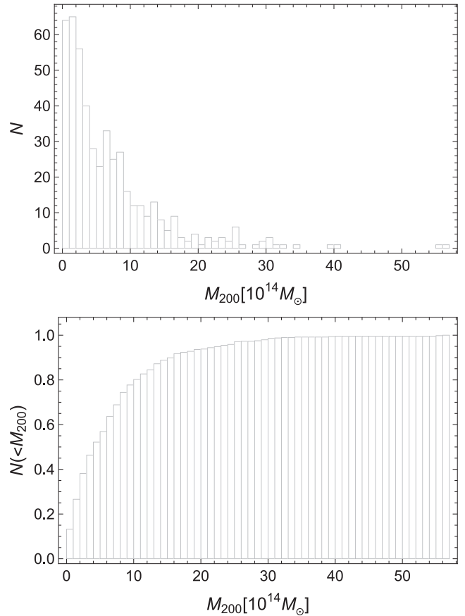
Figure 3. Mass distribution of the 485 WL clusters in the LC^2 -single catalogue. Top panel: Histogram of the mass distribution. Bottom panel: Normalized cumulative function. M_{200} is in units of 10^{14} M_\odot .
