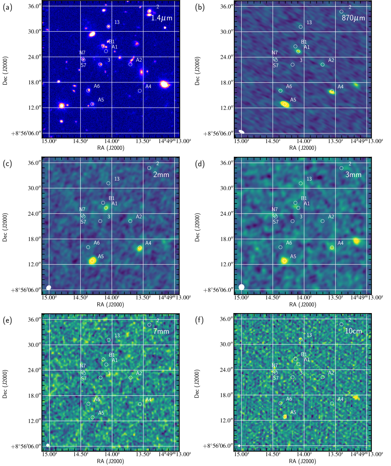
Figure 1. Continuum images of Cl J1449+0856: (a) near infra-red 1.4\mu\text{m} (HST/WFC3), (b) 870\mu\text{m} (ALMA), (c)-(d) 2mm and 3mm (ALMA), (e)-(f) 7mm and 10cm (JVLA). Any line emission present has not been removed from the images. The signal-to-noise of the galaxies can be seen to decrease towards the longer wavelengths. In the 10cm image, only the deep, high-resolution A-configuration data is shown, without the C-configuration. The images have not been corrected for the primary beam attenuation of the instruments. The galaxies indicated show the positions of the galaxies for which we find CO[4-3] detections, with the exception of A4 and A5, which are discussed in Section 3.8, and ID 2, which is only detected at 870\mu\text{m} . A bright foreground galaxy can be seen to the West of A4, which has been spectroscopically confirmed at z=1.3 , and will therefore not be discussed in this paper.
