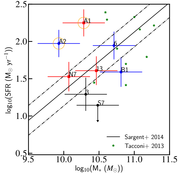
Figure 8. The SFR- M_* plane. The MS of star-forming galaxies at z=2 is shown by the solid black line (Sargent et al. 2014), and a sample of MS galaxies at z \sim 2 are shown by the green stars (Tacconi et al. 2013). The dash-dotted lines represent the 0.2 dex scatter on the MS relation. The cluster galaxies do not show systematic evidence for an increased sSFR with respect to the MS. The errors on the average SFRs include a 0.17 dex systematic uncertainty, in addition to the measurement errors. The colour-coding is as in Fig. 7. The orange empty circles highlight galaxies that have had their stellar masses estimated from their dynamical mass, A1 and A2. 2\sigma upper limits are shown. For S7, the SFR has been calculated using the CO[4-3] line flux only, as we do not believe the measured 870\mu\text{m} flux is associated with S7.
