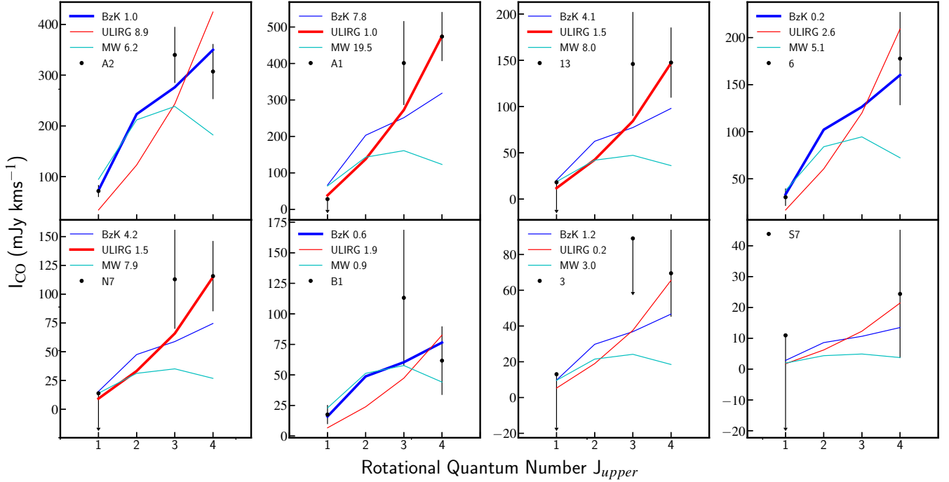
Figure 6. CO SLEDs of 8 cluster galaxies detected in CO[4-3]. The legends show the reduced \chi^2 value for the fits of the observed galaxy CO SLED with the three excitation models: BzK, ULIRG/SB and MW. The SLEDs of some galaxies are best-fit by a BzK excitation model, and some are best-fit by a ULIRG/starburst-like model. The preferred template for each galaxy is plot with a thicker line, where possible. We do not draw any conclusions about the gas excitation of galaxies ID 3 and S7, due to the limited data available. A least-squared analysis was used for the fitting, and 2\sigma flux upper limits are shown.
