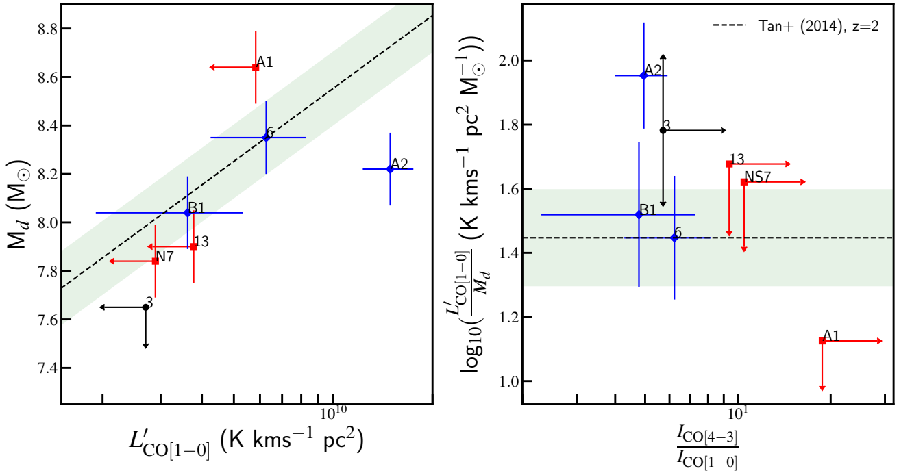
Figure 11. Left: Dust mass against L'_{CO[1-0]} . The expected MS trend from Tan et al. (2014) is shown by the black dashed line in both panels. The green bands represent the \pm 0.15 dex scatter on the relations, from Daddi et al. (2010a). Right: \frac{L'_{CO[1-0]}}{M_d} as a function of excitation ratio. The galaxies scatter around the expected relation, with the possible exception of A1, discussed in the text. The symbol colour-coding is as in Fig. 7. 2\sigma upper limits are shown.
