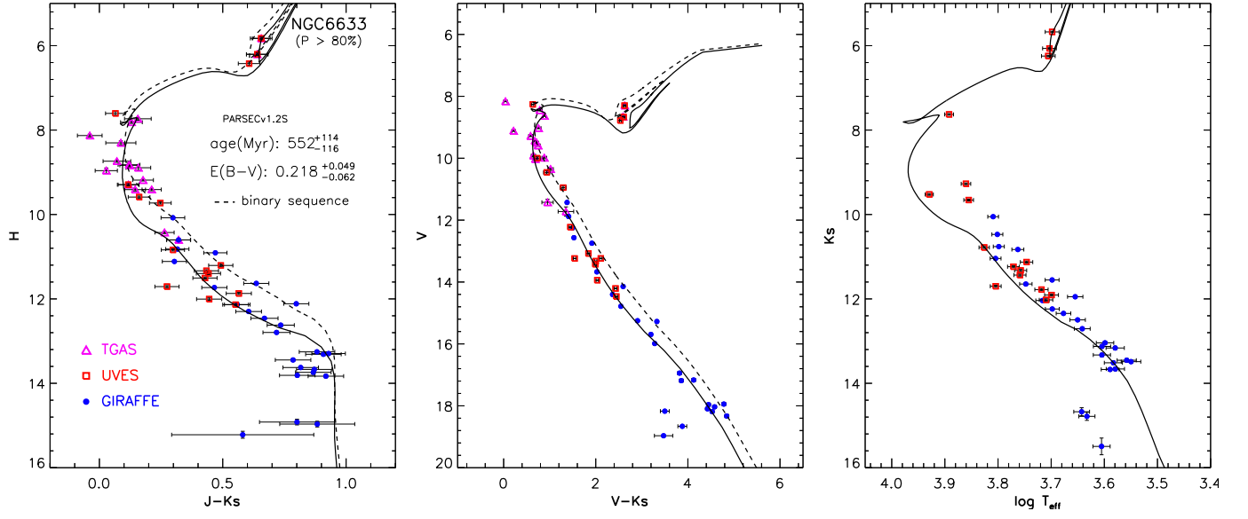
Fig. C.3. As in Fig. 7, but for the cluster NGC 6633 with the PARSEC isochrones.
