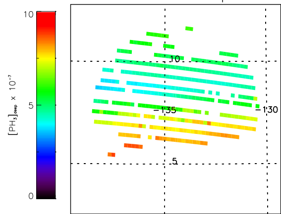
160826_225716 Phosphine
