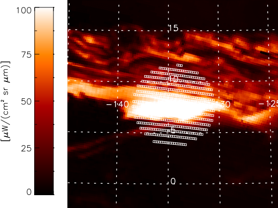
160826_225716 Mean Radiance in M-Filter
