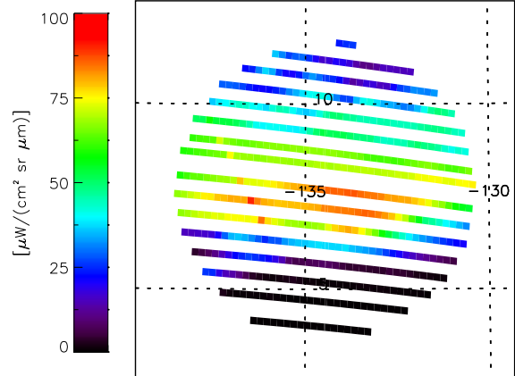
160826_225716 Observed radiance @ 4.996 \mu m
