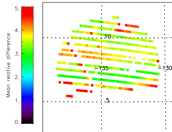
160826_225716 Fit
