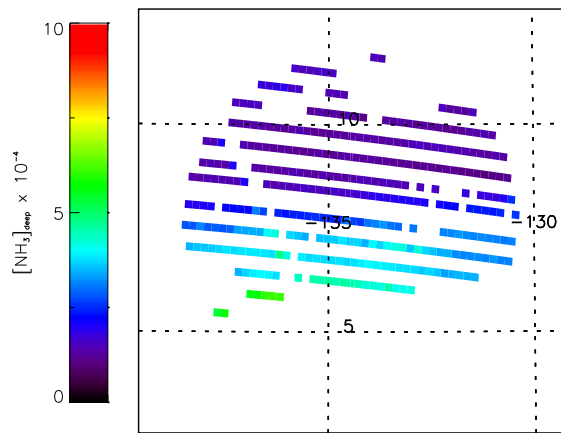
160826_225716 Ammonia
