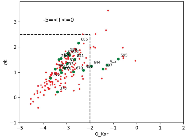
Fig. 2. Degree of isolation of the observed sample (green circles) over-plotted on all iETGs (red circles) in the AMIGA sample. According to Verley et al. (2007a), the horizontal and vertical dashed lines enclose the fiducial range of isolated galaxies in the AMIGA sample.
