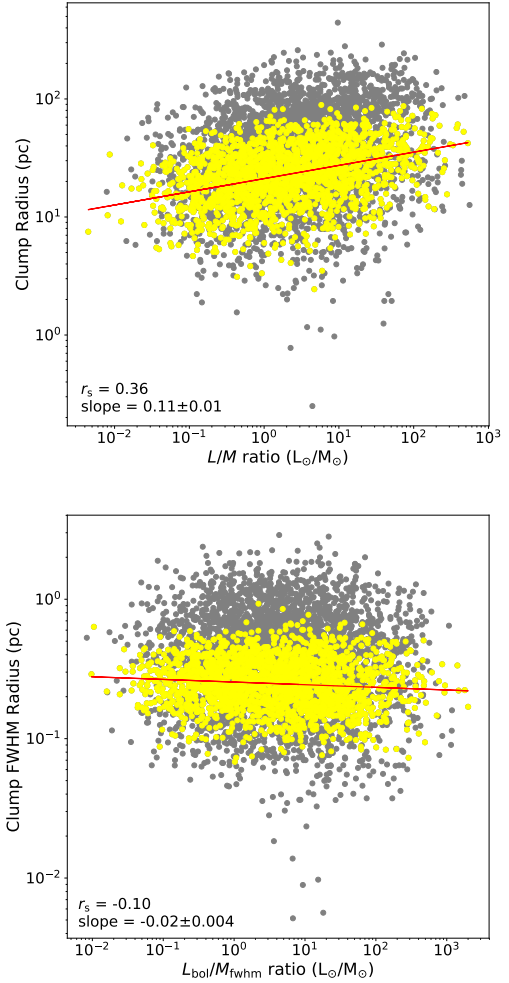
Figure 9. The upper panel presents the clump radius vs clump LM ratio for previously calculated values of radius, luminosity and mass within the ATLASGAL survey. The lower panel presents clump FWHM radius against clump L_{\text{bol}}/M_{\text{fwhm}} ratio, for the newly derived clump sizes (see Sect. 4.2). Both plots present the entire ATLASGAL sample and a distance limited sample (2 to 4 kpc) in grey and yellow respectively. The results from a Spearman's rank correlation coefficient test for the distance limited samples (2 to 4 kpc) is shown in the lower left of each panel, the p -value for both distributions is below our significance threshold.
