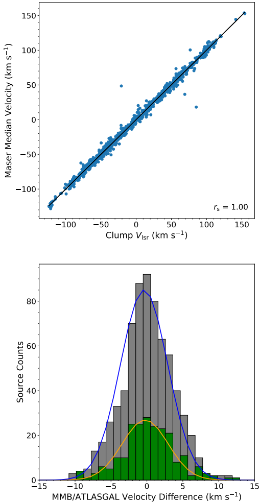
Figure 5. The upper panel presents the distribution of the median maser velocities against the clump velocities for the entire matched sample ( 60^\circ \leq \ell \leq 186^\circ ), with a best fit line shown. The results from a Spearman's rank correlation test is shown in the lower right of the plot. The lower panel presents histograms of the offsets between the median maser velocities and the molecular line velocities for every match in the MMB survey is shown in grey with the matches for the latest addition to the MMB survey shown in green. Gaussian curves have been fitted to the data to determine the mean and standard deviations of the distributions.
