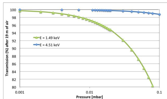
Figure 1: Transmission of X-ray photons of 4.51 keV and 1.49 keV, along the 19 m vacuum tube of BEaTriX, as a function of residual vacuum pressure
