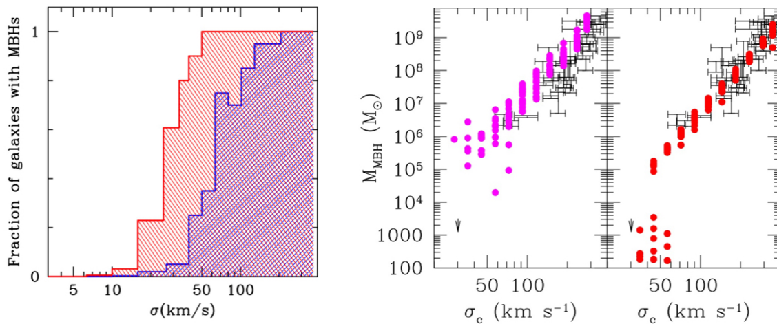
Figure 1. Predictions at z = 0 from the models of Volonteri et al. (2008b) and van Wassenhove et al. (2010) provide diagnostics for distinguishing between BH seed formation mechanisms. The observational signatures of BH seeds are strongest in dwarf galaxies. Left: BH occupation fraction as a function of velocity dispersion for light seeds (remnants from Pop III stars; red) and heavy seeds (direct collapse; purple). Courtesy of M. Volonteri. Right: M_{\text{BH}} - \sigma relation at z = 0 starting with heavy (purple, left panel) and light (red, right panel) seeds. Observational data (black points) are from Tremaine et al. (2002). Adapted from Volonteri et al. (2008a).
