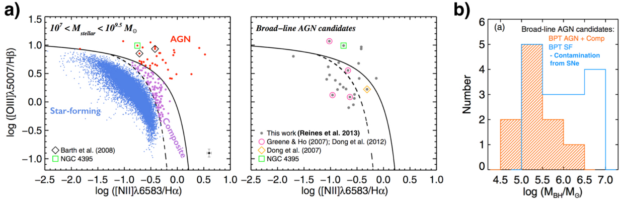
Figure 12. Optical signatures of active massive BHs in dwarf galaxies adapted from Reines et al. (2013). a) BPT diagram for \sim 25,000 dwarf emission line galaxies in the SDSS with M_\star \lesssim 3 \times 10^9 M_\odot and z < 0.055 . 35 objects fall in the AGN part of the diagram (red points) and 101 objects fall in the “composite” (AGN+SF) part of the diagram (purple points). Of these 136 dwarf galaxies with narrow-line signatures indicating an active massive BH, 10 have broad H\alpha emission likely signifying dense gas orbiting close to the BH. An additional 15 galaxies in the star-forming part of the BPT diagram exhibit broad H\alpha emission in their spectra. b) Distribution of BH masses for the galaxies with broad H\alpha emission in their SDSS spectra. BH masses are calculated using equation 5 in Reines et al. (2013), which is based on the method of Greene & Ho (2005) but uses the updated radius-luminosity relationship of Bentz et al. (2013). The apparent excess at larger BH masses for the BPT star-forming objects (blue histogram) is most likely due to SNe masquerading as broad-line AGN (e.g., Baldassare et al. 2016a). For the more secure broad-line AGN candidates (BPT AGN + composites; orange histogram), the median BH mass is just \langle M_{\text{BH}} \rangle \sim 2 \times 10^5 M_\odot . All 10 of the broad-line AGN and composites are also detected in X-rays with Chandra (Baldassare et al. 2016b). © AAS. Reproduced with permission.
