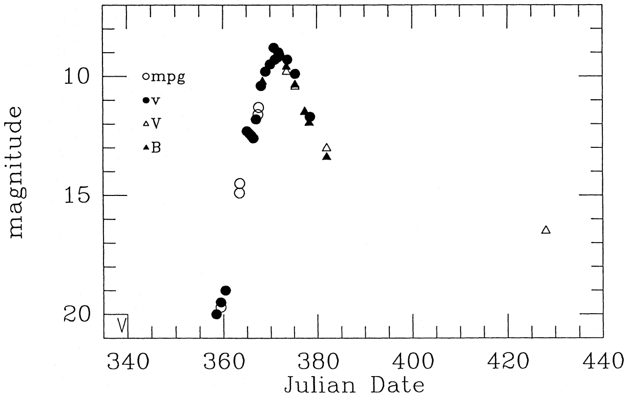
Fig. 1. Lightcurve of nova LMC 1991. Magnitudes derived from the IAU Cirrs. The two last points arise from observations obtained with the 3.6m telescope at La Silla.
