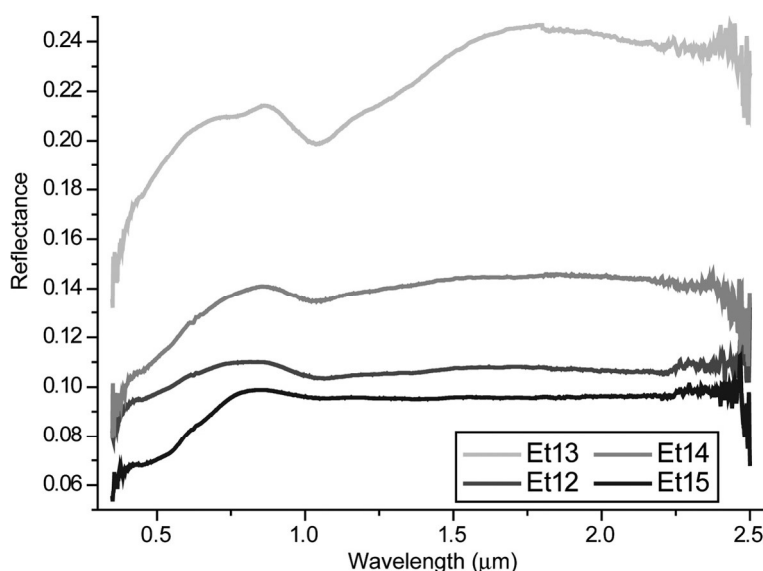
Fig. 5. Spectra of four different samples from a Mount Etna lava flow. The samples have very similar P.I., with similar relative mineral associations, but with different groundmass textures. The intensity of the C.F. composite band, which is due to mafic and pl mineralogy, is strongly reduced from sample Et13 to Et15, increasing the tachylitic glass content in the groundmass of these samples (see also Fig. 6 and Tables 2 & 3). These spectra were acquired with a FieldspecPro® i = 30^\circ , e = 0^\circ , white Spectralon standard Labsphere®, QTH lamp, at SLAB, IAPS-INAF, Rome.
