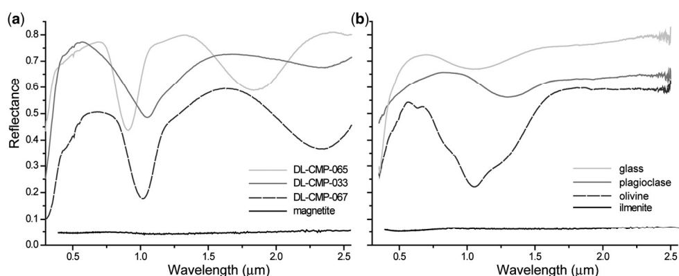
Fig. 1. Examples of mineral spectra. (a) pxs (opx DL-CMP-065, En 90 ; cpx DL-CMP-067, Wo 39 En 52 and DL-CMP-033, Wo 49 En 42 ; particle size <40 µm) from Klima–RELAB library and magnetite from the USGS mineral library. (b) Anorthositic glass (FeO 1.8 wt%, g.s. particle size 20–50 µm; Carli et al. 2013), plagioclase (An 80 , FeO 0.5 wt%, 36–63 µm; Serventi et al. 2013a), olivine (Fo 88 , 36–63 µm; Serventi et al. 2013a) and ilmenite from the USGS library. In this box, the reflectance is shifted for clarity as follows: glass +0.1, pl +0.5 and ol –0.5.
