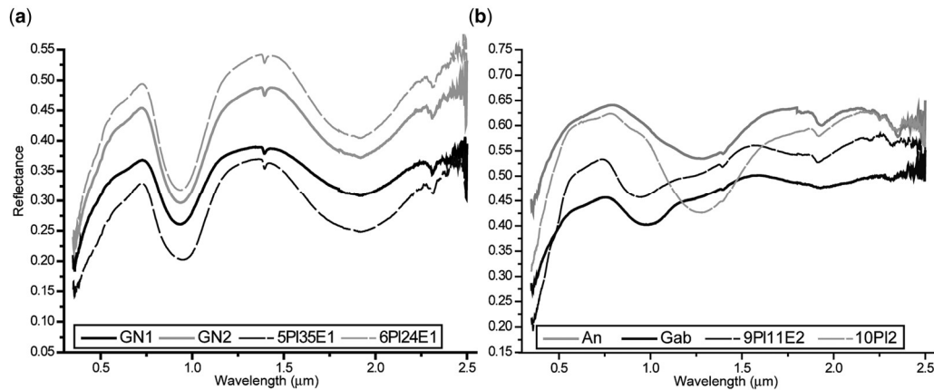
Fig. 2. An example of reflectance spectra from mineral mixtures, with particle size 250–125 \mu\text{m} (Serventi et al. 2013b), and rock powders, with grain size < 250 \mu\text{m} (Carli 2009). Left box: GN1 55% pl (An80–FeO 0.36 wt%); 10% cpx (En 44 Wo 46 ); 35% opx (En 75 ); GN2 61% pl (An81–FeO 0.37 wt%); 17% cpx (En 46 Wo 45 ); 22% opx (En 78 ). These samples are spectrally similar (e.g. position and intensity) to mineral mixtures 5PI35E1 and 6PI24E1, respectively (50% Pl3, 50% E1 and 60% Pl2, 40% E1, see Serventi et al. 2013b). Right box: An (94% pl (An79–FeO 0.45 wt%), 4% cpx (En 42 Wo 45 ); Gab (81% pl (An79–FeO 0.36 wt%), 16% cpx (En 42 Wo 45 ); 3% opx (En 82 )). These samples are spectrally similar (e.g. in terms of position and intensity) to mineral mixtures 10PI2 and 9PI11E2, respectively (100% Pl2 and 90% Pl1, 10% E2; see Serventi et al. 2013b). For clarity, the reflectance of the 6PI24E1 and An spectra have been shifted, by +2.5% and 5%, respectively.
