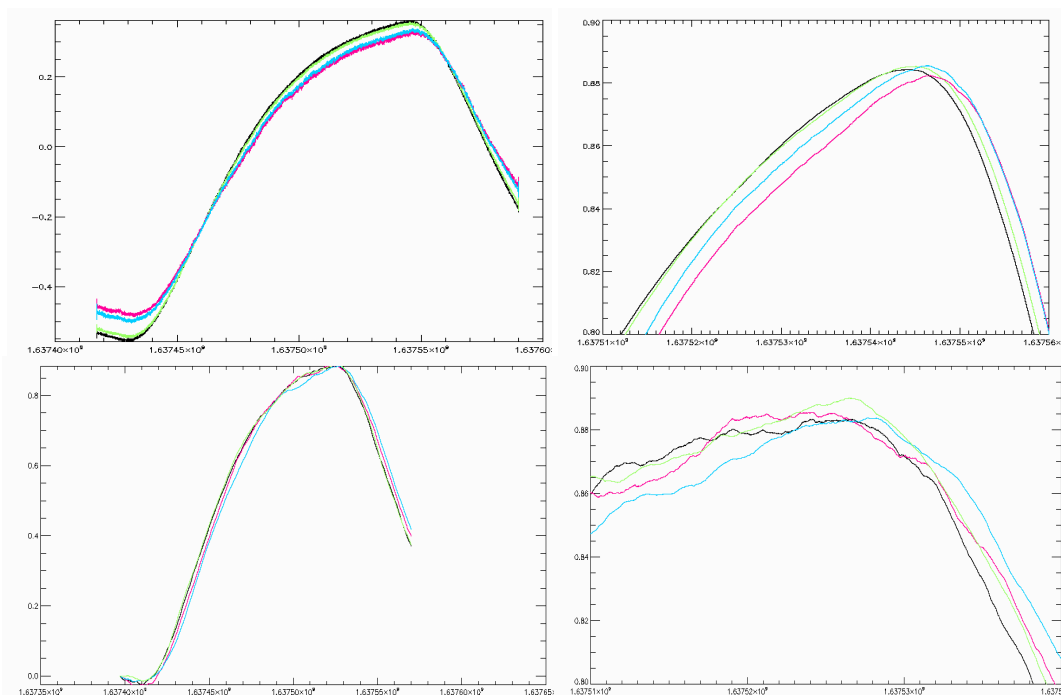
Figure 3 Top Left: An overall plot of the back end temperature rise event between the ODs 191 and 193. Curves are smoothed and mean subtracted: black is R_BEM1, green R_BEM2, light blue is L_BEM1, purple L_BEM2. Top Right: curves are further filtered and normalized in order to have a similar height around the peak. Bottom Left and Right: normalized curves of sky outputs of RCAs color coded the same way of the sensors on top plots by physical proximity: black is RCA28-01, green RCA26-11, purple is RCA27-11 and light blue is RCA25-01
