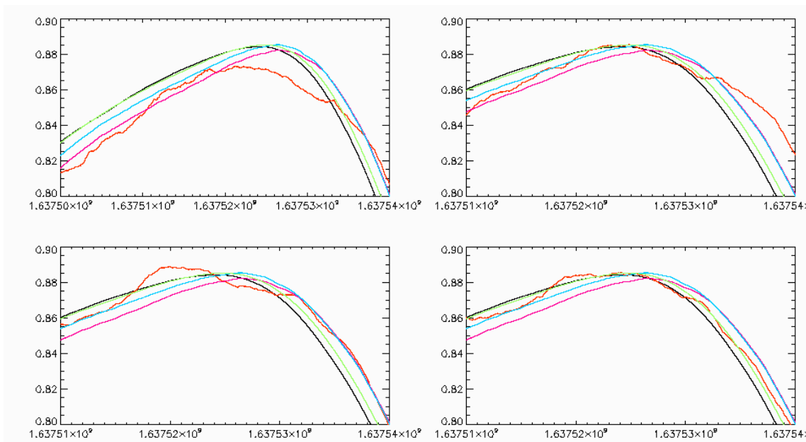
Figure 6 Smoothed sensors (black is R\_BEM1 , green R\_BEM2 , purple is L\_BEM1 , light blue L\_BEM2 ) in the same peaked region than Figure 3 are compared with RCA27 detectors signal output (red). Top left is detector M-00, top right M-01, bottom left is S-10, bottom right S-11.
