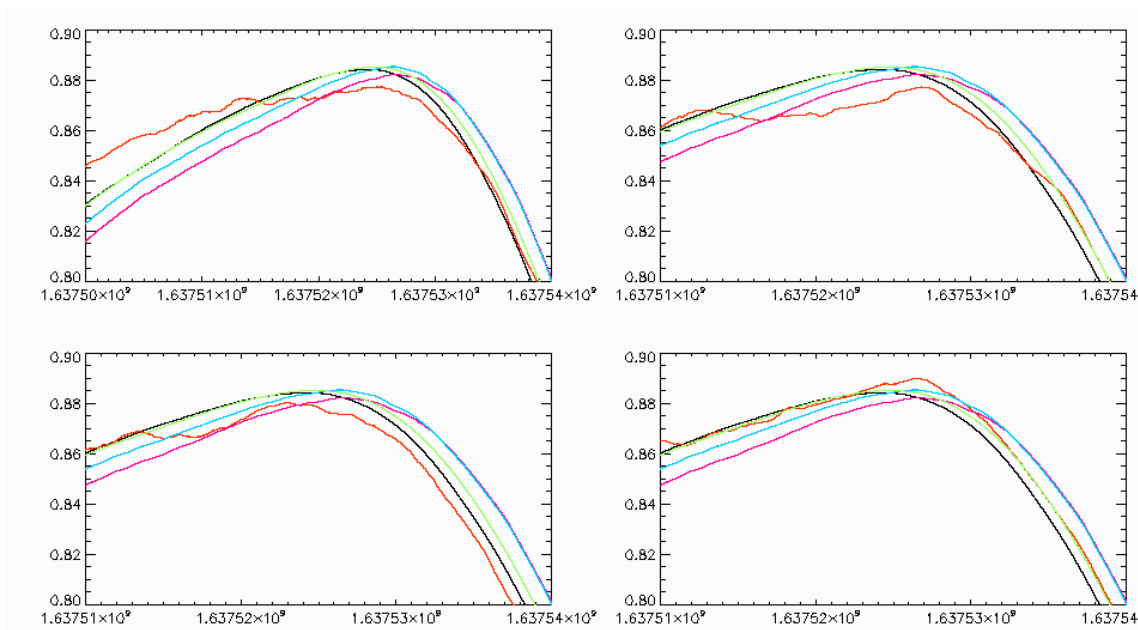
Figure 5 Smoothed sensors (black is R\_BEM1 , green R\_BEM2 , purple is L\_BEM1 , light blue L\_BEM2 ) in the same peaked region than Figure 3 are compared with RCA26 detectors signal output (red). Top left is detector M-00, top right M-01, bottom left is S-10, bottom right S-11.
