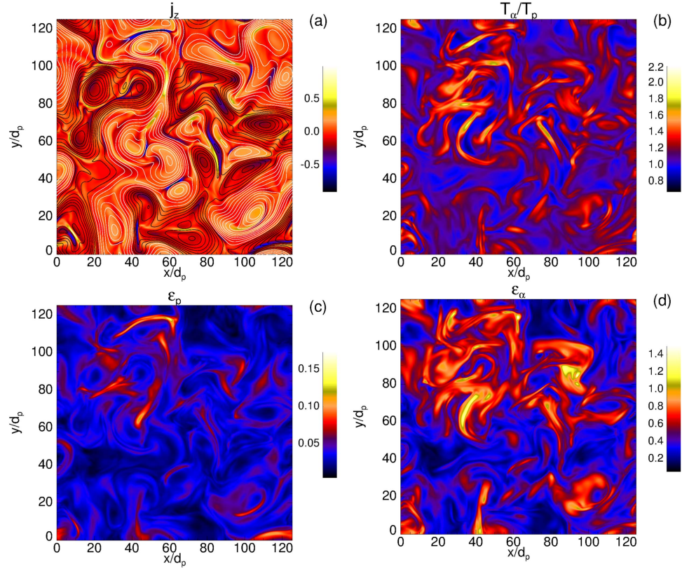
Figure 4. (a) Out of plane current density j_z . The isolines of the magnetic potential A_z are indicated by (black/white) lines. (b) Ratio between alpha particle and proton temperatures. Panels (c) and (d): \epsilon for both protons and alpha particles, respectively. Each contour map is at the maximum of the turbulent activity.
