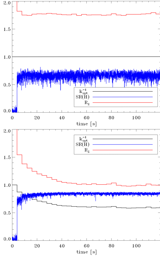
Fig. 7. Results of numerical simulations showing the performance (SR at 1.65\ \mu\text{m} , blue line) when NCPA correction is applied. Top: OGTL is off ( k_{\text{opt}} fixed to 1, black line) and the SR shows values dispersed in the interval 0.5–0.8, with an average value of 0.67. R_z indicates a clear overcorrection of the NCPA. The corresponding long exposure PSF on the scientific arm is shown in the center image of Fig. 6. Bottom: OGTL is active, the SR reaches an average value of 0.87, and R_z converges to 1. The long exposure PSF on the scientific arm is shown in the right panel of Fig. 6.
