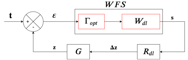
Fig. 2. Block diagram reports the main elements of the considered AO loop. The wavefront sensor block is made up of two parts: W_{dl} and \Gamma_{opt} . This last time-dependent diagonal matrix takes into account the WFS modal sensitivity variations due to a change in the closed-loop wavefront residuals.
