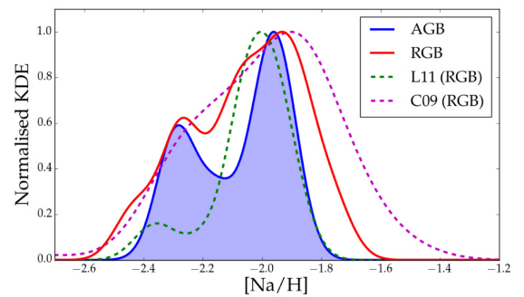
Figure 7. Gaussian KDEs of our NGC 6397 [\text{Na/H}] abundances, along with those of L11 and Carretta et al. (2009a, C09), with systematic offsets removed (see the text for details). A smoothing bandwidth of 0.06 dex (total Na uncertainty, see Table 7) was applied to each of our RGB and AGB data sets, while for C09 we used a bandwidth of 0.11 dex, matching their total error calculations (see C09, Appendix A). L11 did not quote total abundance uncertainties, however their average measurement uncertainty in Na was the same as in our sample (0.04 dex), therefore we applied an identical bandwidth of 0.06 dex. The discrepancy between the relative heights of the two peaks in the L11 sample, compared to those of the other samples, may be due to the low number of stars observed in L11 (21 RGB stars).
