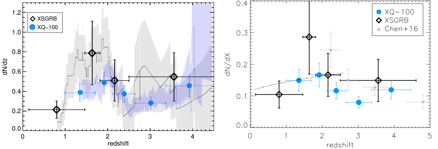
Fig. 3. Left hand panel: incidence rates from the two legacy samples of strong Mg II absorbers with points representing bin sizes with 6 and 20 absorbers in the XSGRB and XQ-100 samples, respectively. The grey line illustrates a sliding redshift binning of XSGRB absorbers and the shaded region presents the 68% confidence levels. The blue shaded region represents the 68% confidence intervals for a similar sliding redshift binning of the XQ-100 sample. Right hand panel: comoving line density. The dotted line represent strong Mg II absorbers in quasar spectra (Mathes et al. 2017), and the grey stars mark a larger sample of quasar absorbers at high redshifts (Chen et al. 2016).
