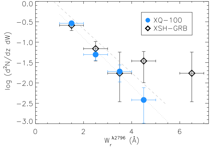
Fig. 5. The equivalent width distribution of W_r^{2796} of the GRB and quasar samples. Vertical error bars were computed using the \sqrt{N_{\text{abs}}} approximation. The dotted and dashed lines represent best fits for the distribution of quasar absorbers by Mathes et al. (2017) and Chen et al. (2016), respectively.
