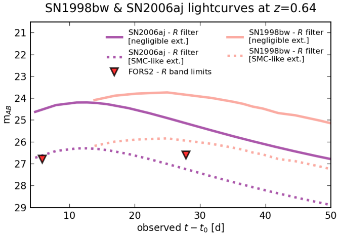
Fig. 20. R -band lightcurves of SN1998bw and SN2006aj placed at the photometric redshift of GRB 211106A. The light curves considering both no extinction and A_V = 2.6 (from Laskar et al. 2022) are shown.
